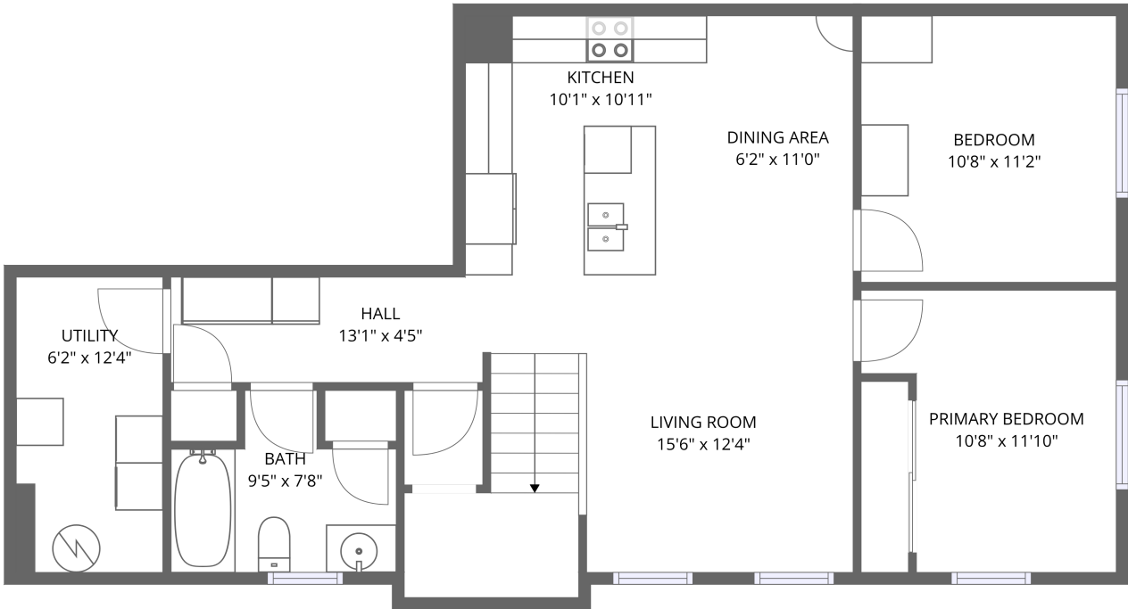
FLOOR 1
