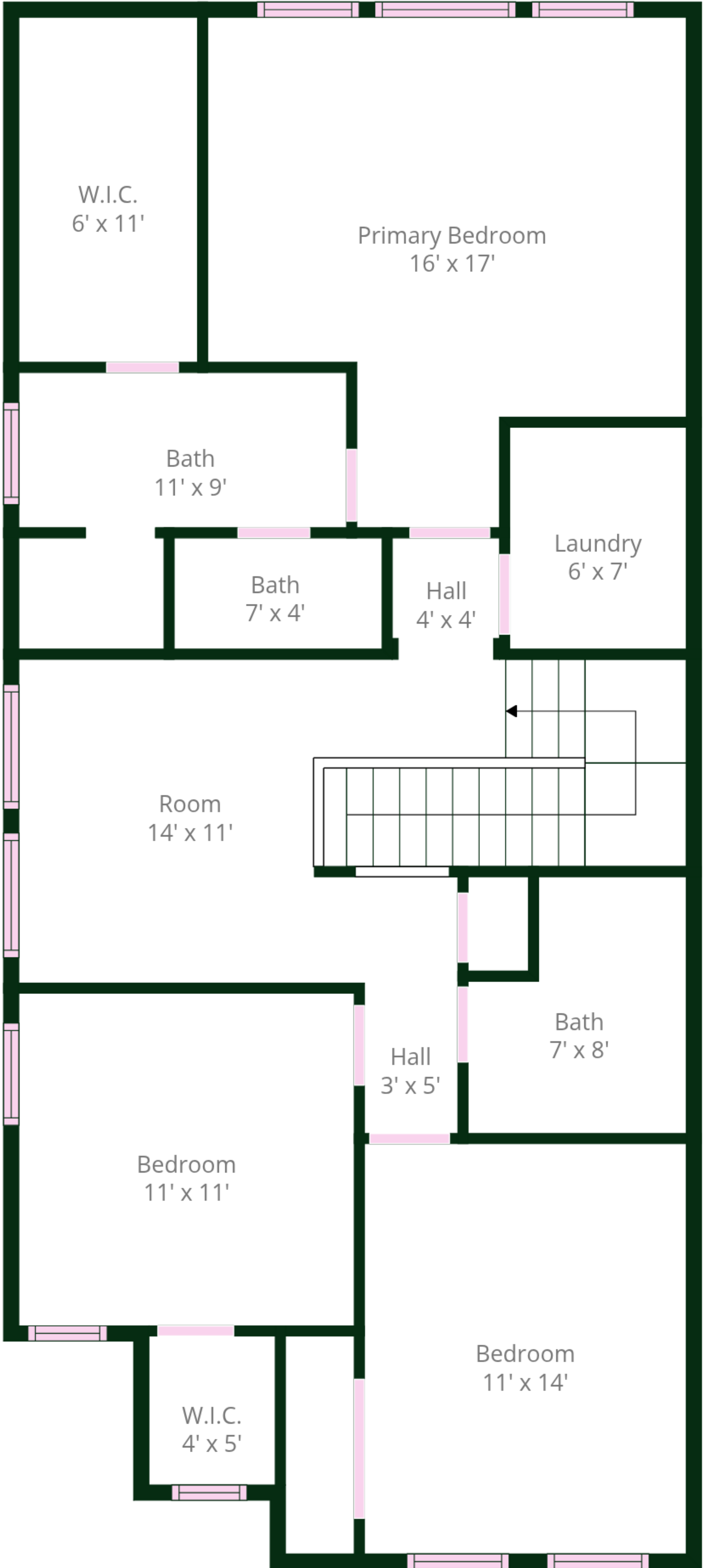
Floor 2
