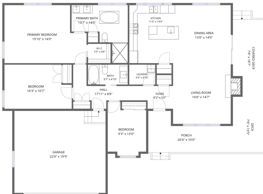
1st floor
