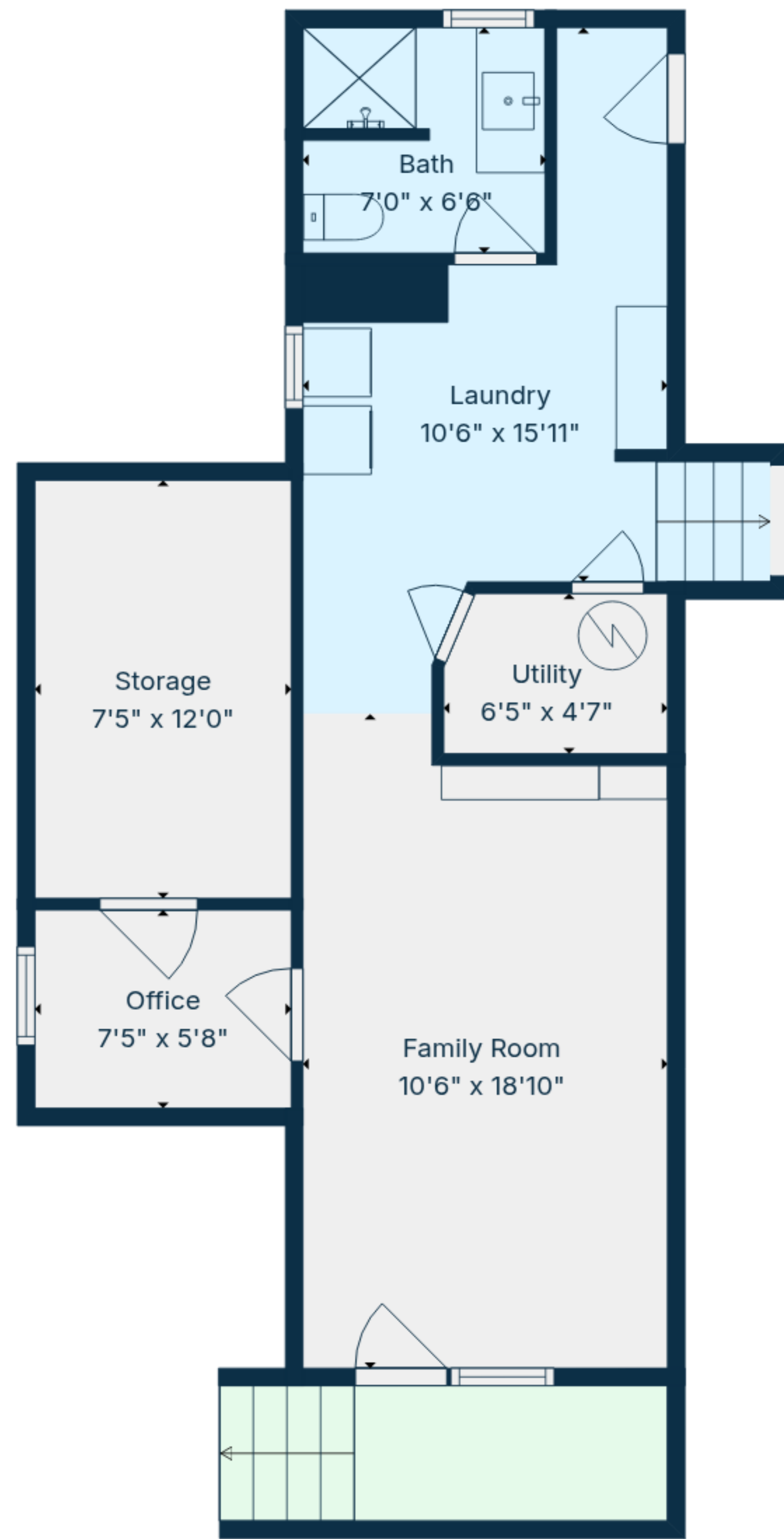
1st Floor
