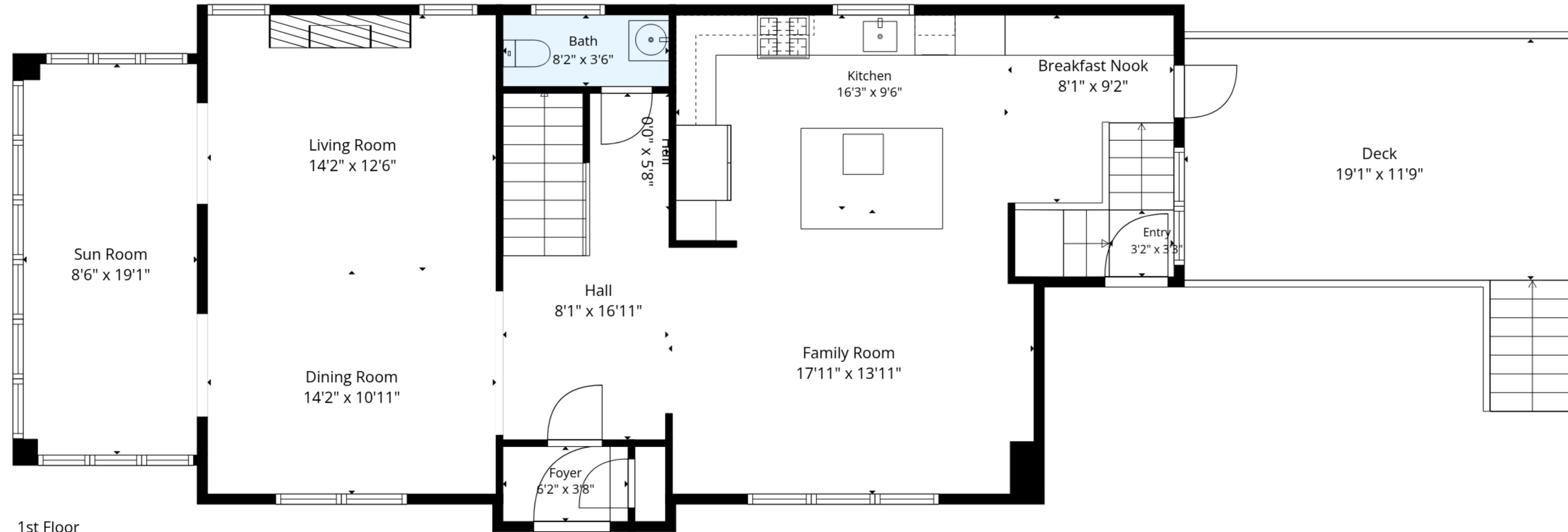
1st Floor
