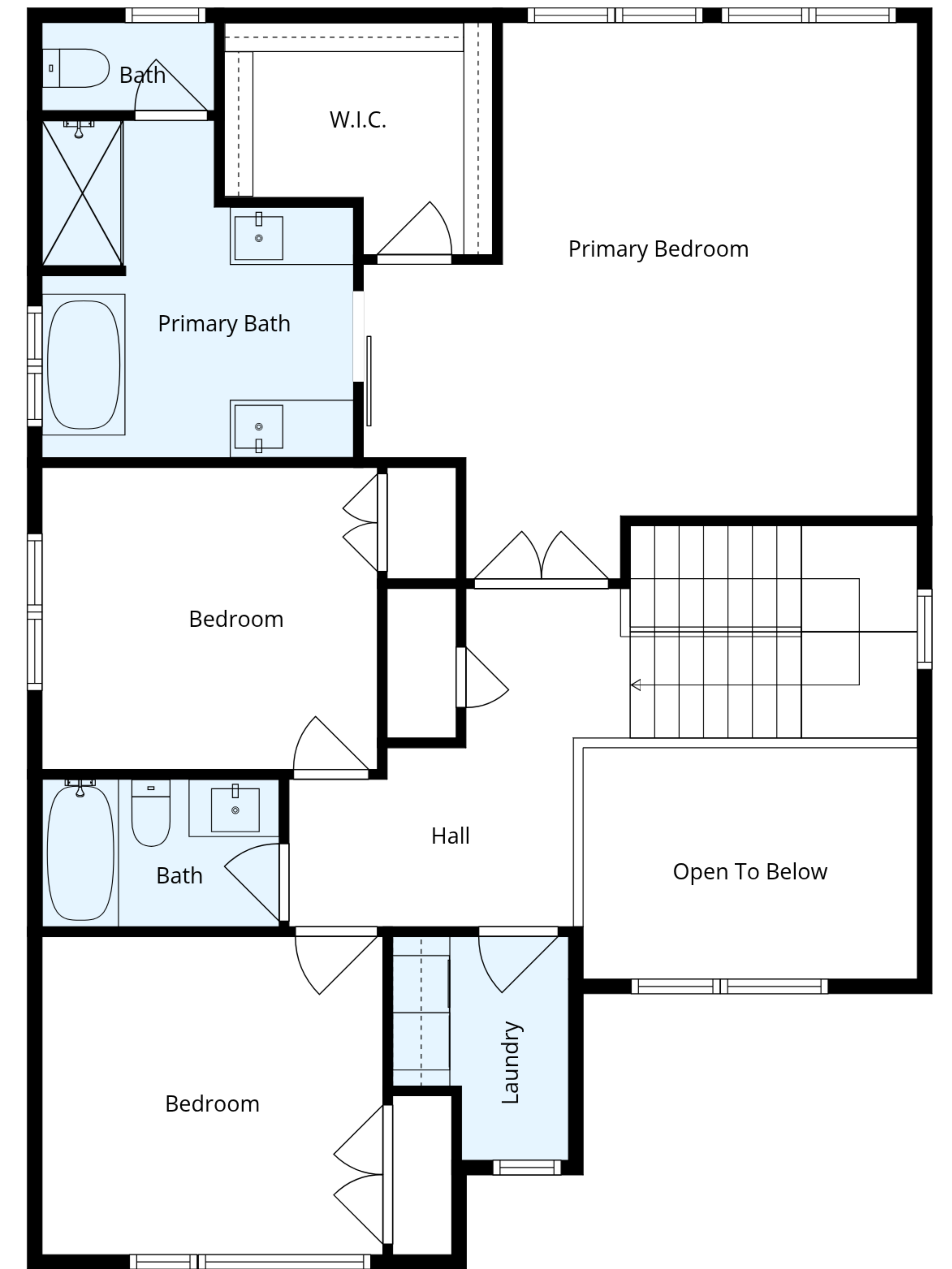
2nd Floor
