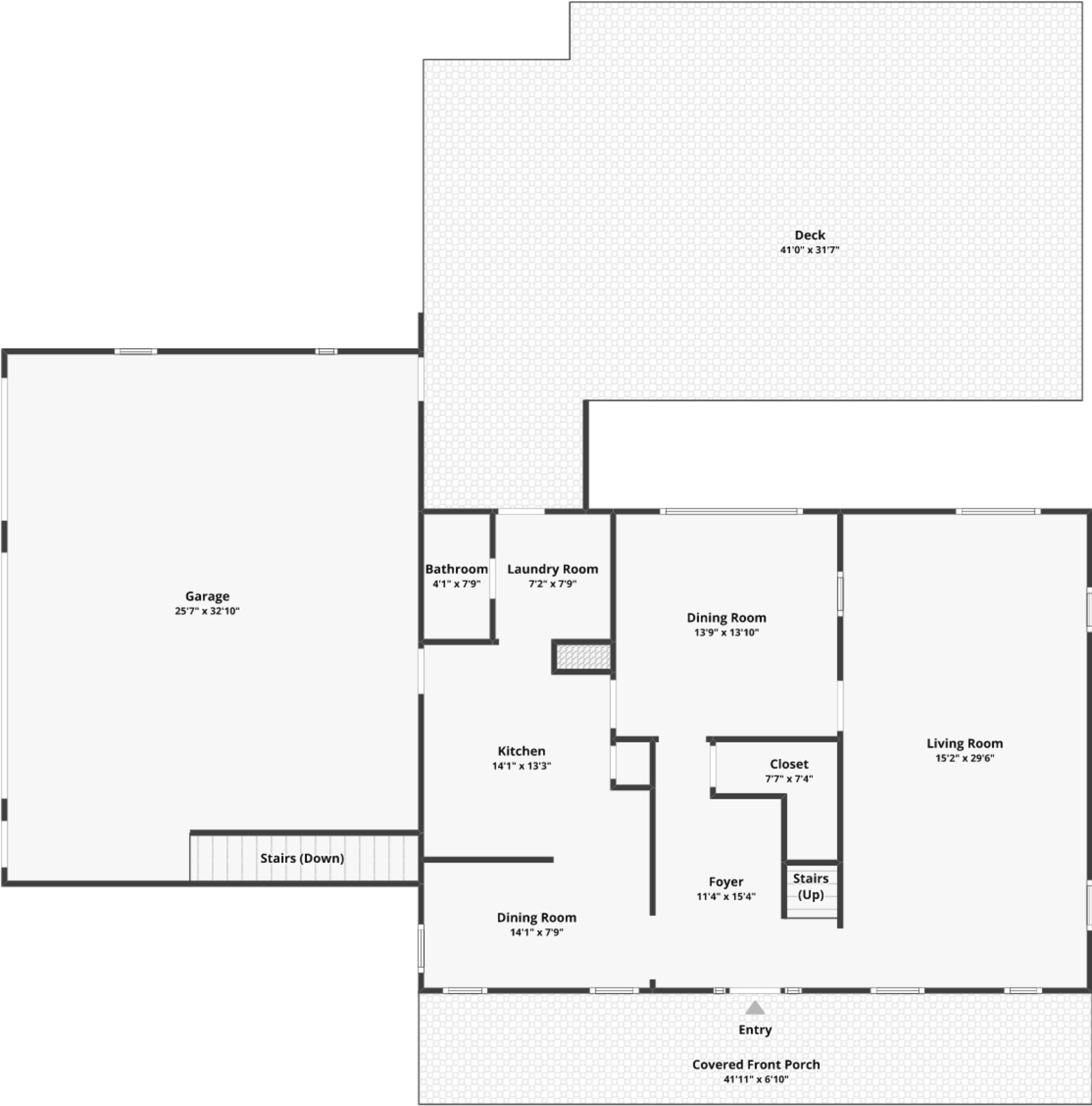
FLOOR 1 Finished area: ~1,200.91 sq. ft. Unfinished area: ~4.94 sq. ft.
