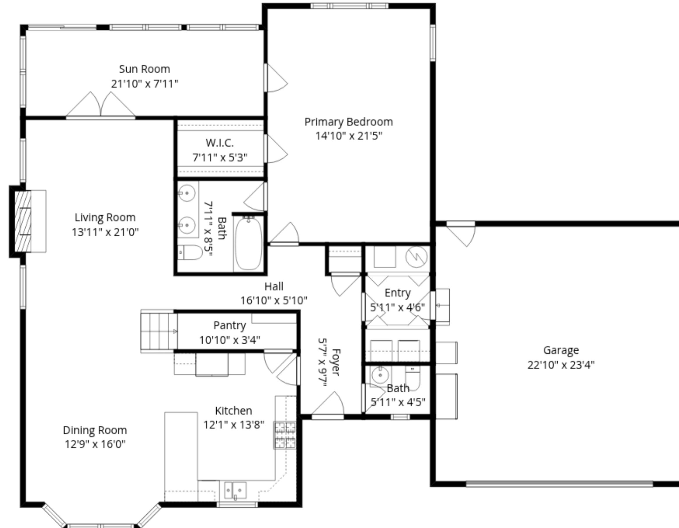
Main Floor
