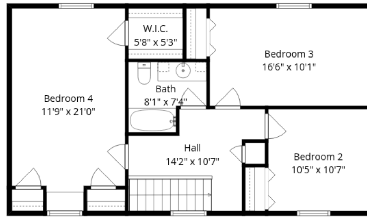
Upper Floor
