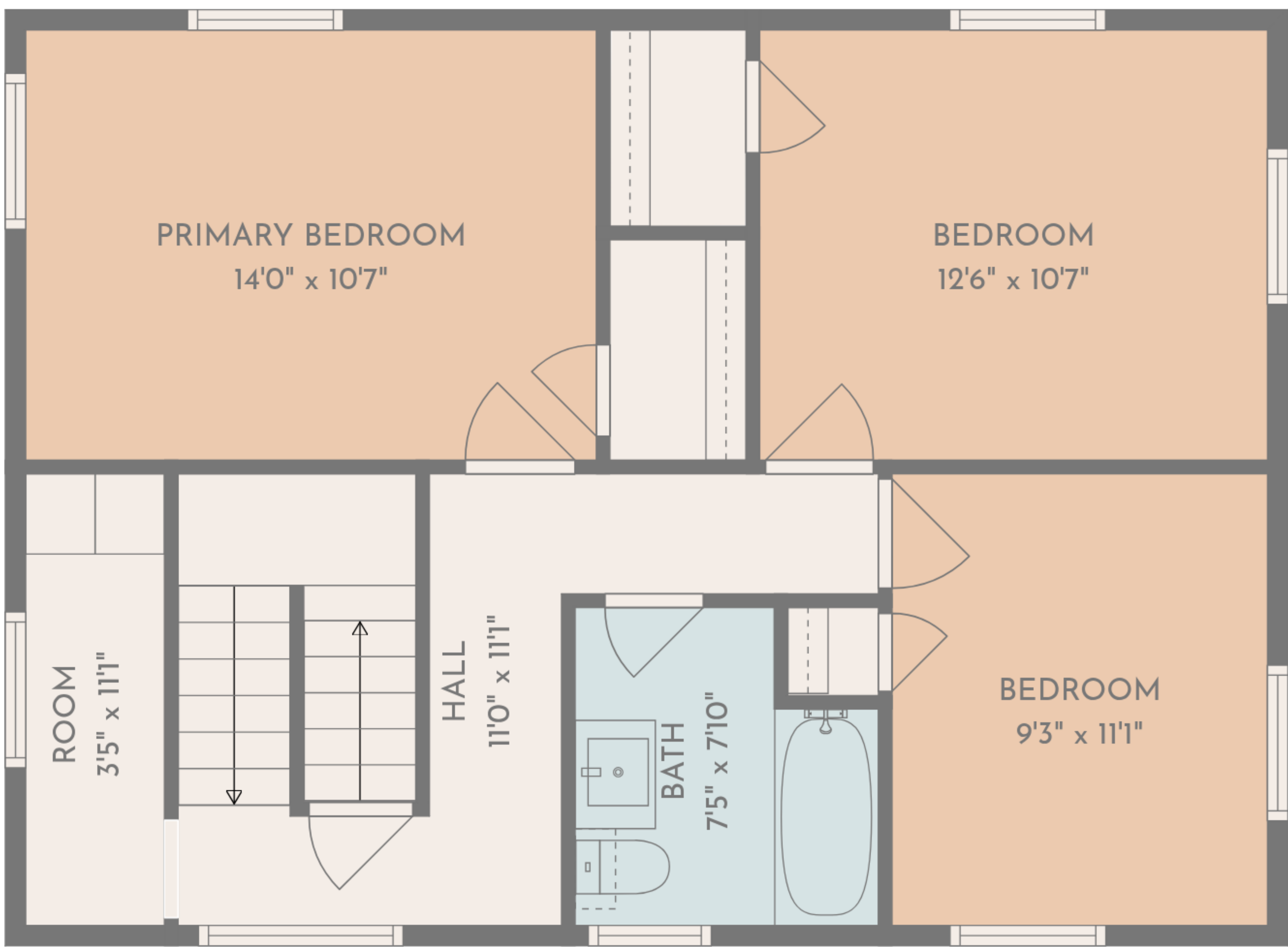
2nd floor
