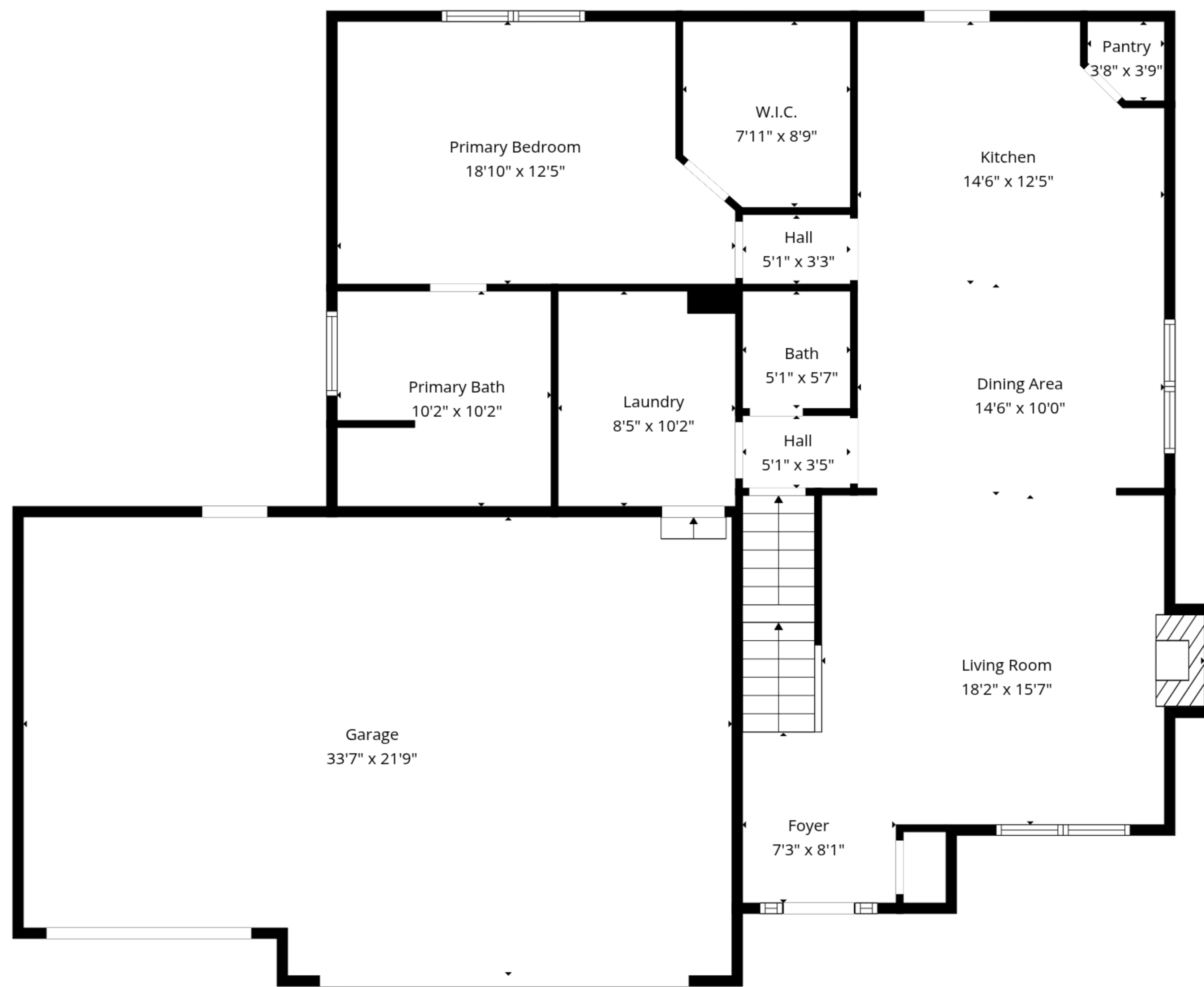
1st Floor
