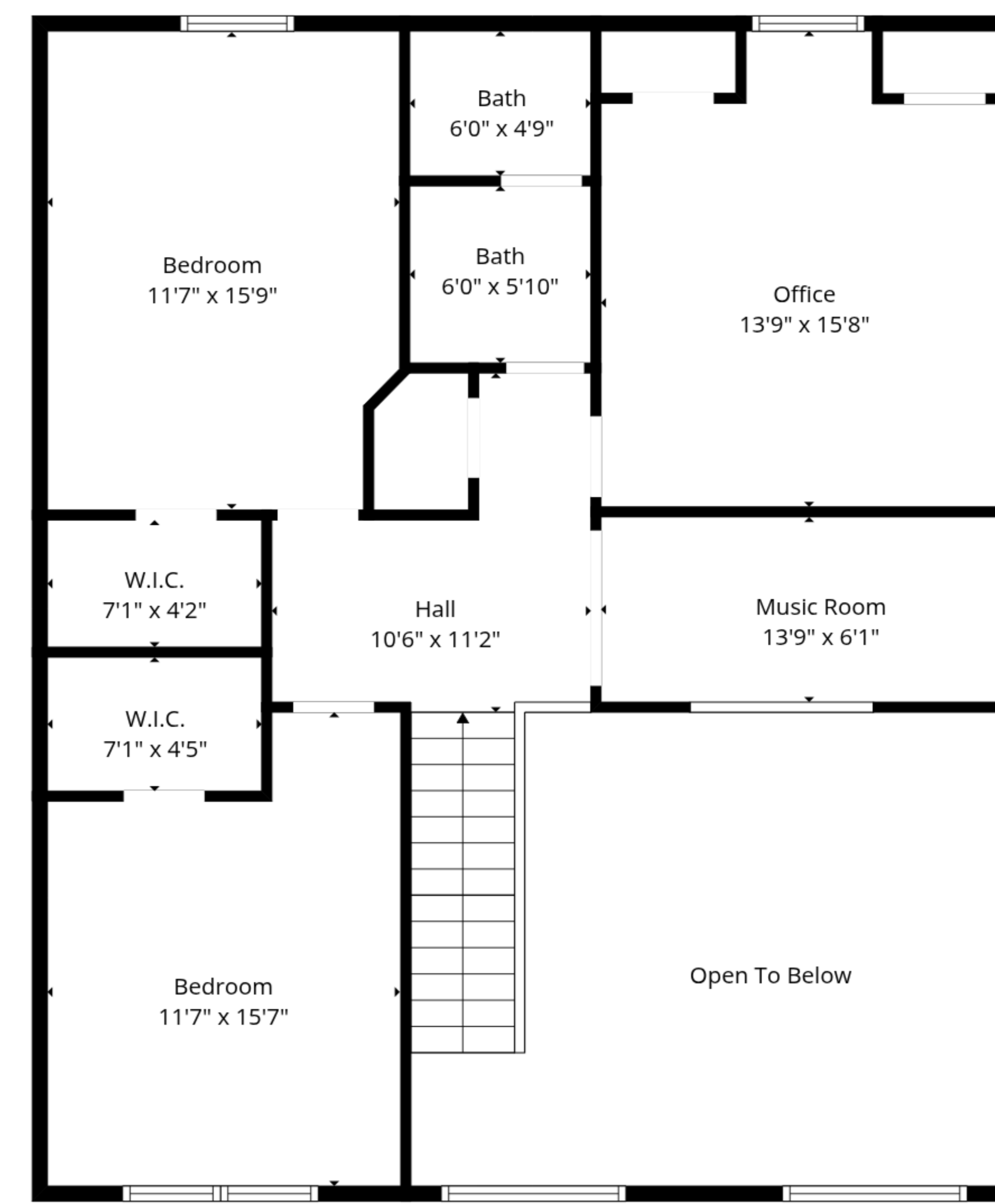
2nd Floor
