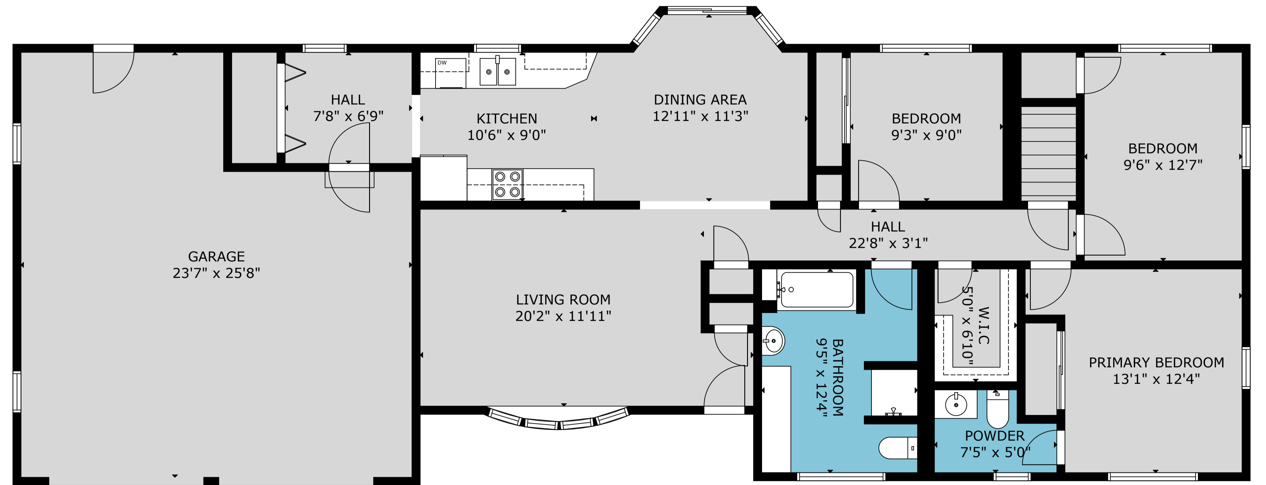
MAIN FLOOR
