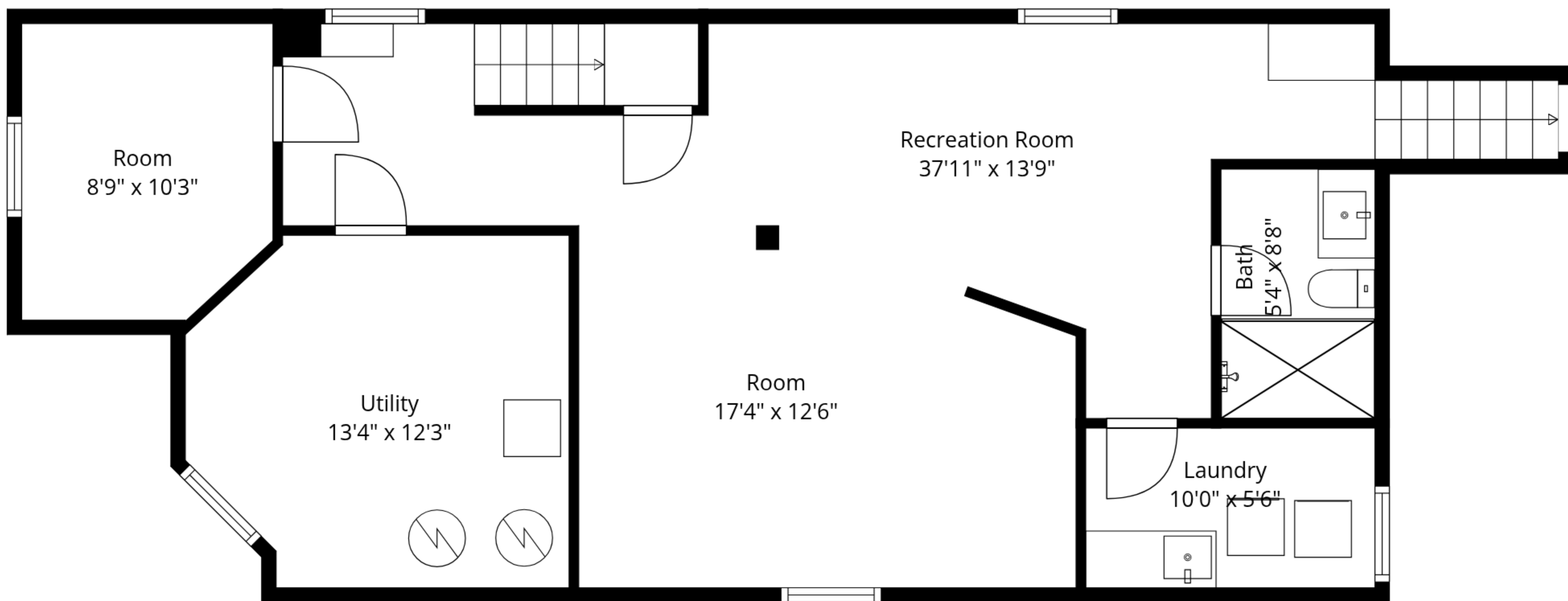
1st Floor
