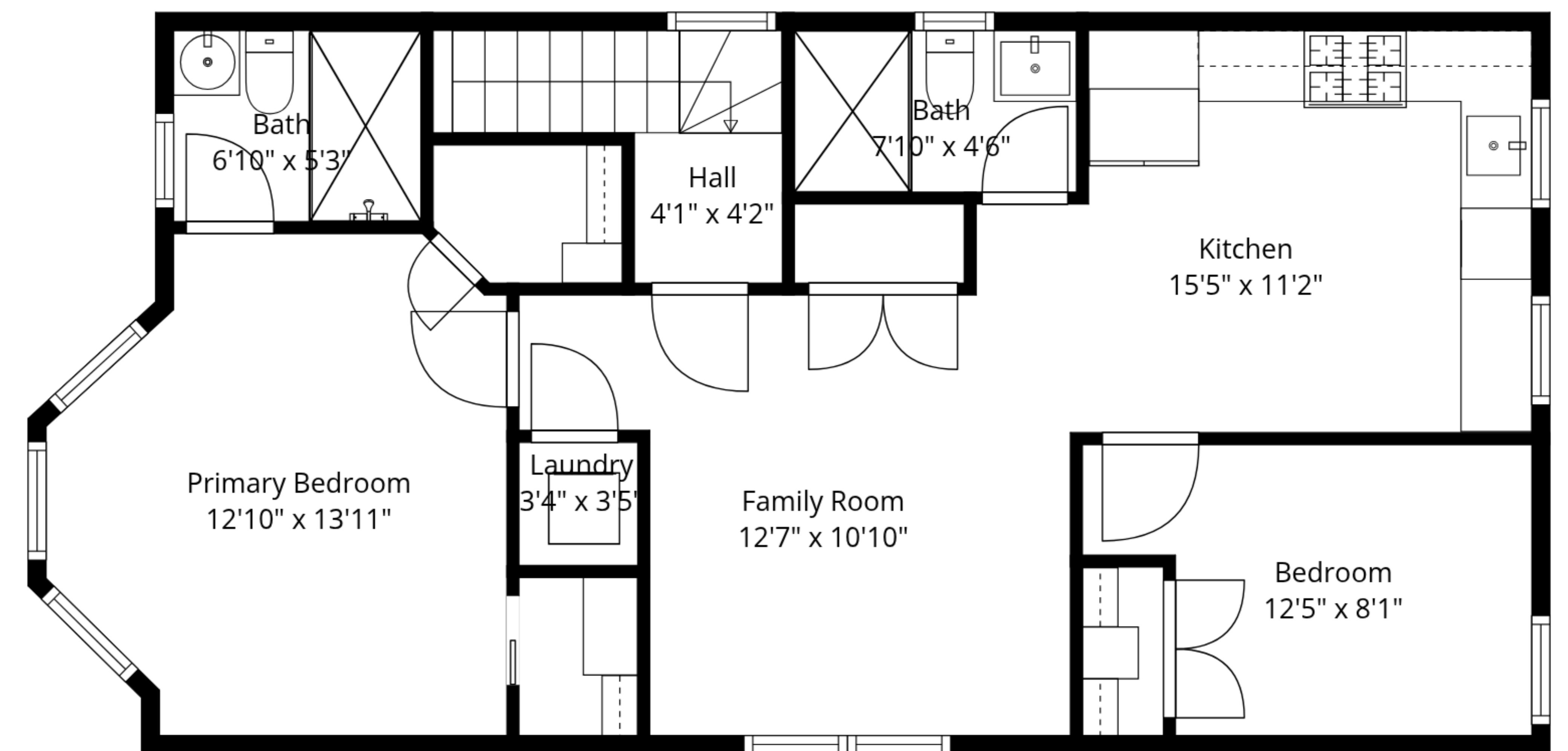
3rd Floor
