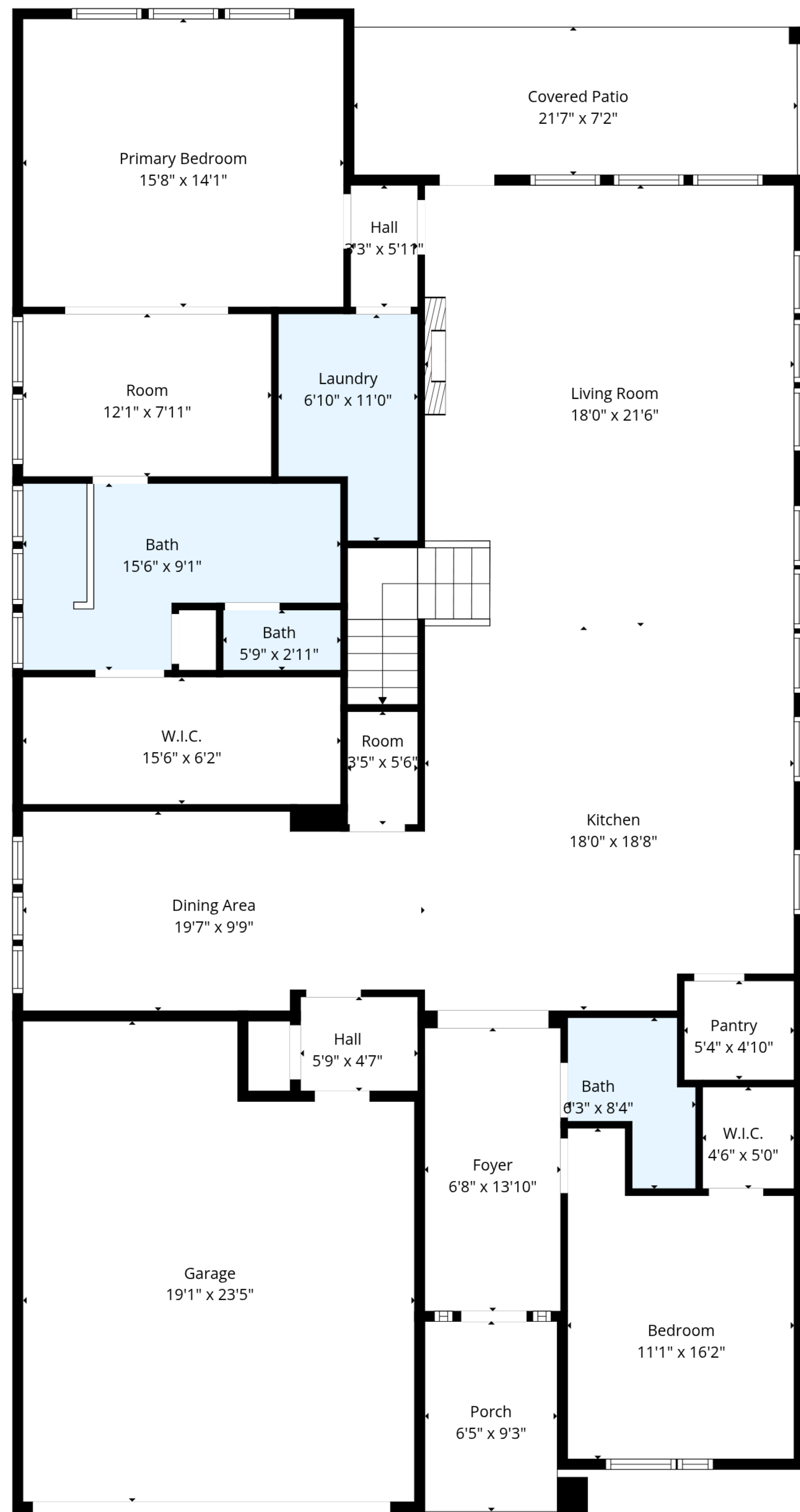
1st Floor
