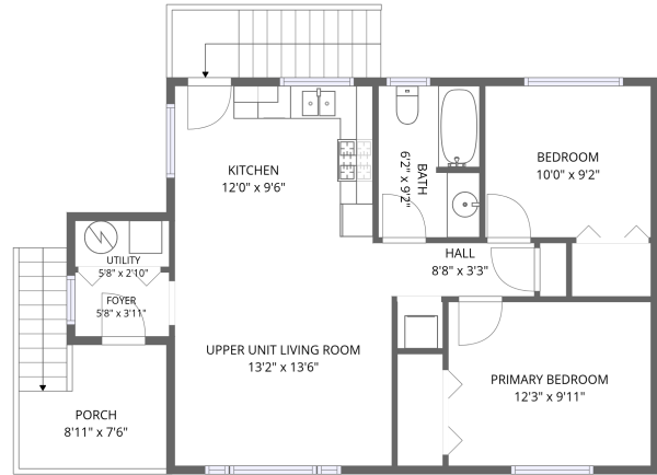
2nd floor
