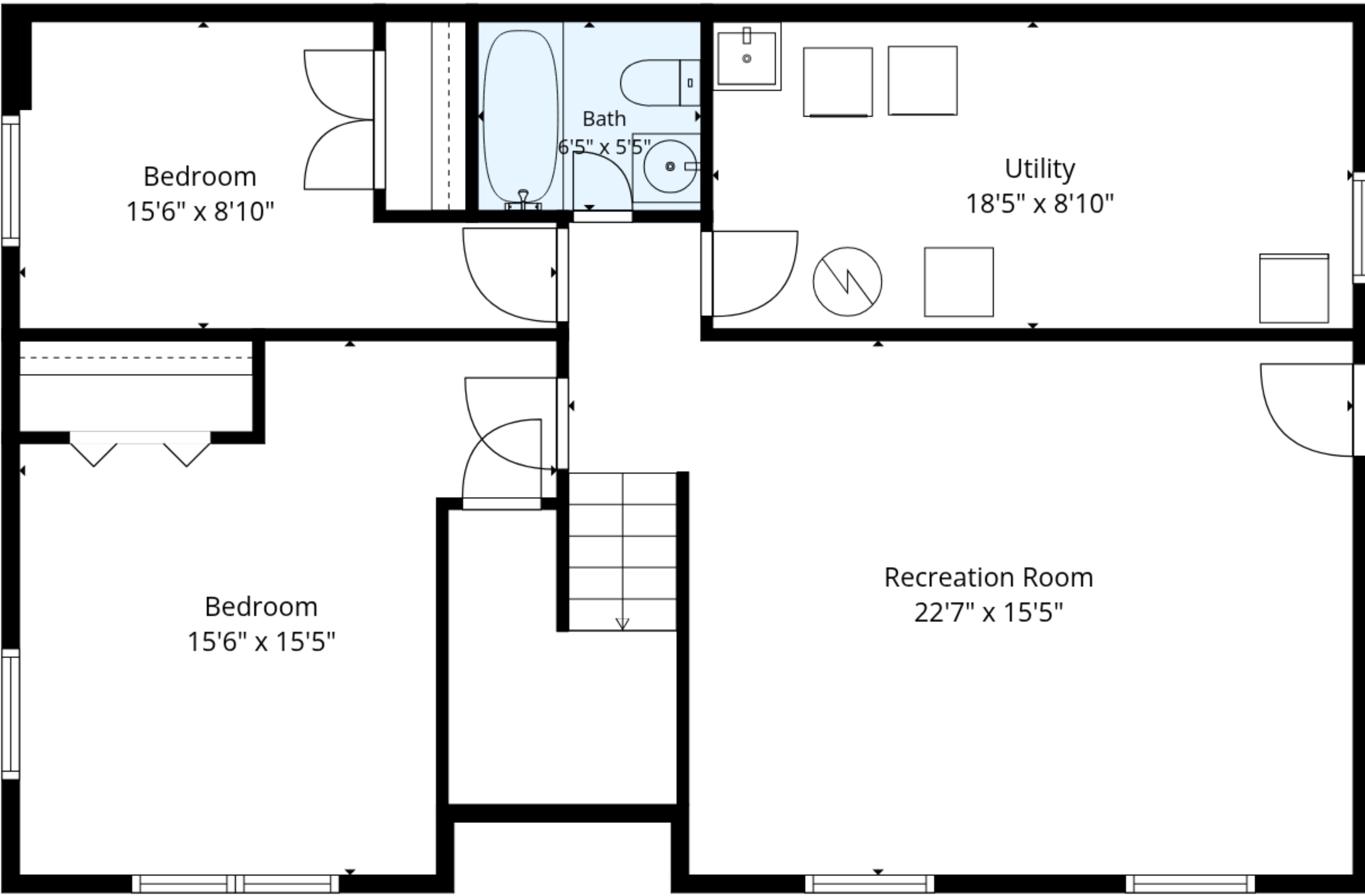
Basement
