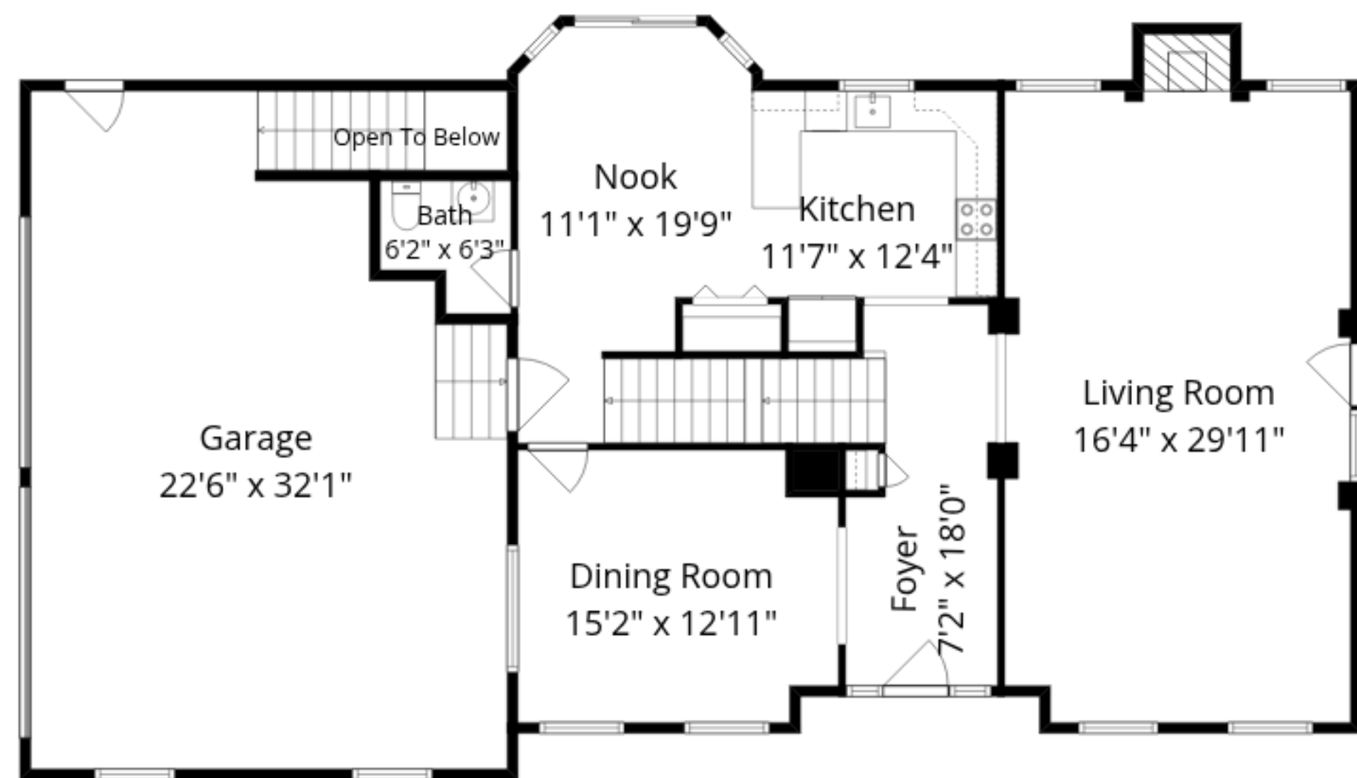
Main Floor
