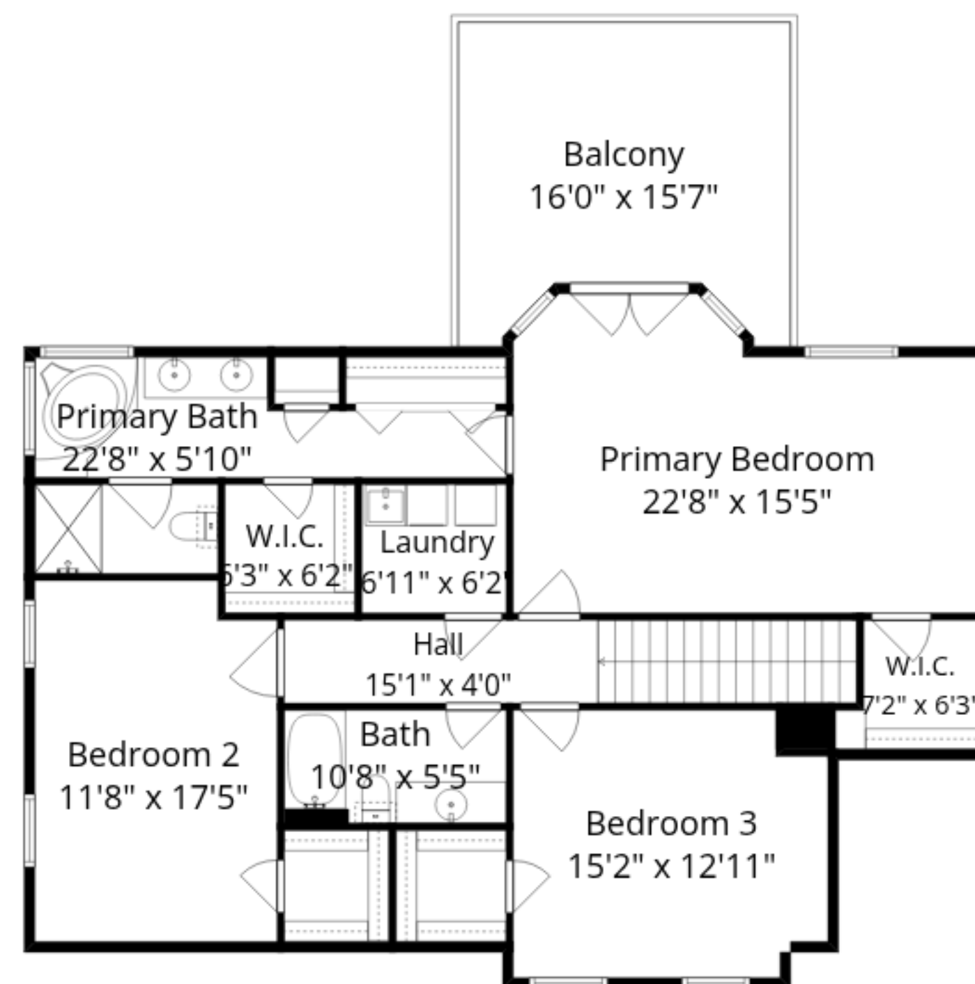
Upper Floor
