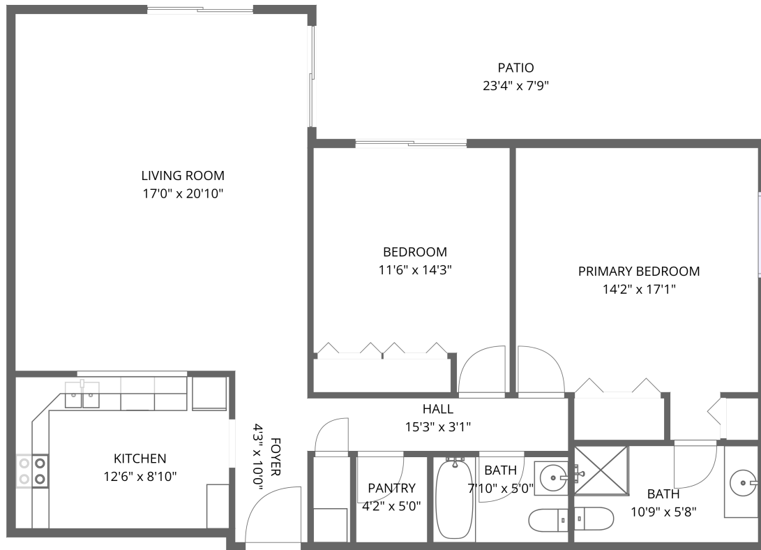
1st floor
