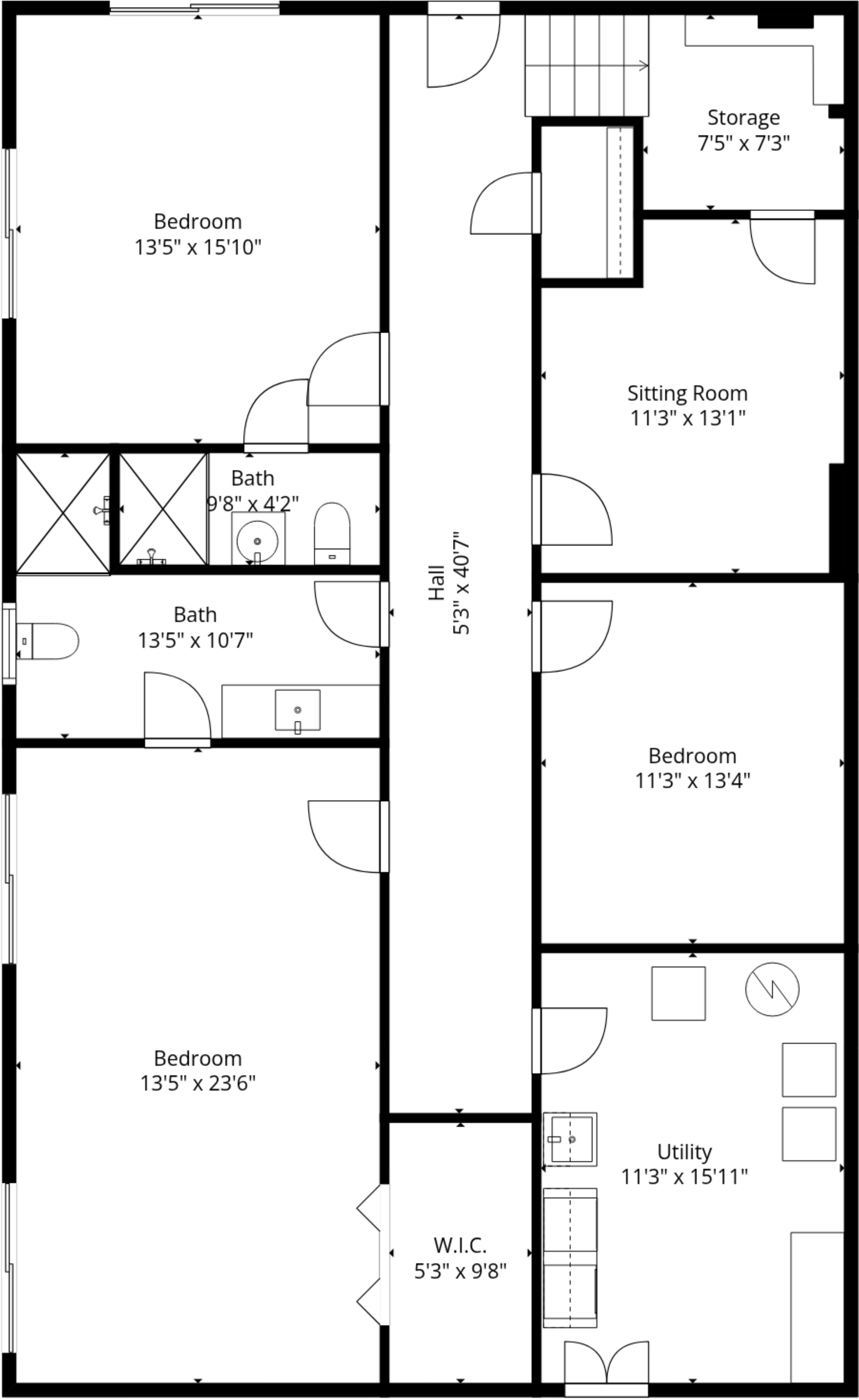
Floor 1
