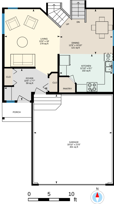
Main Floor Exterior Area 564.73 sq ft
