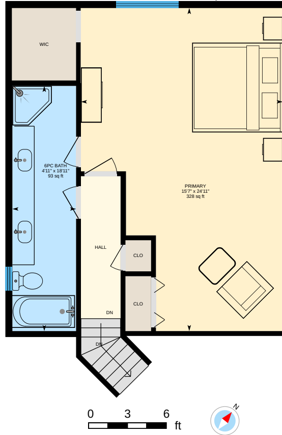
2nd Floor Exterior Area 587.33 sq ft
