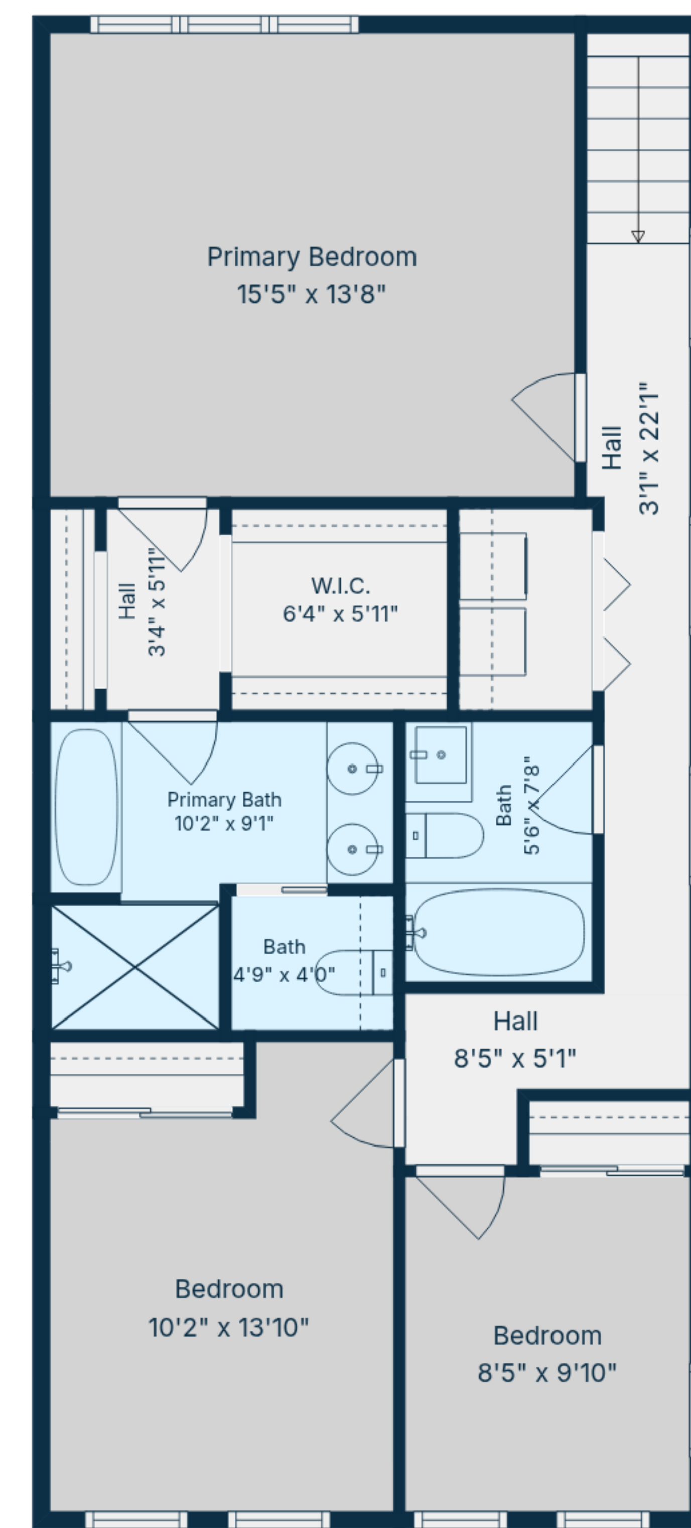
5th Floor
