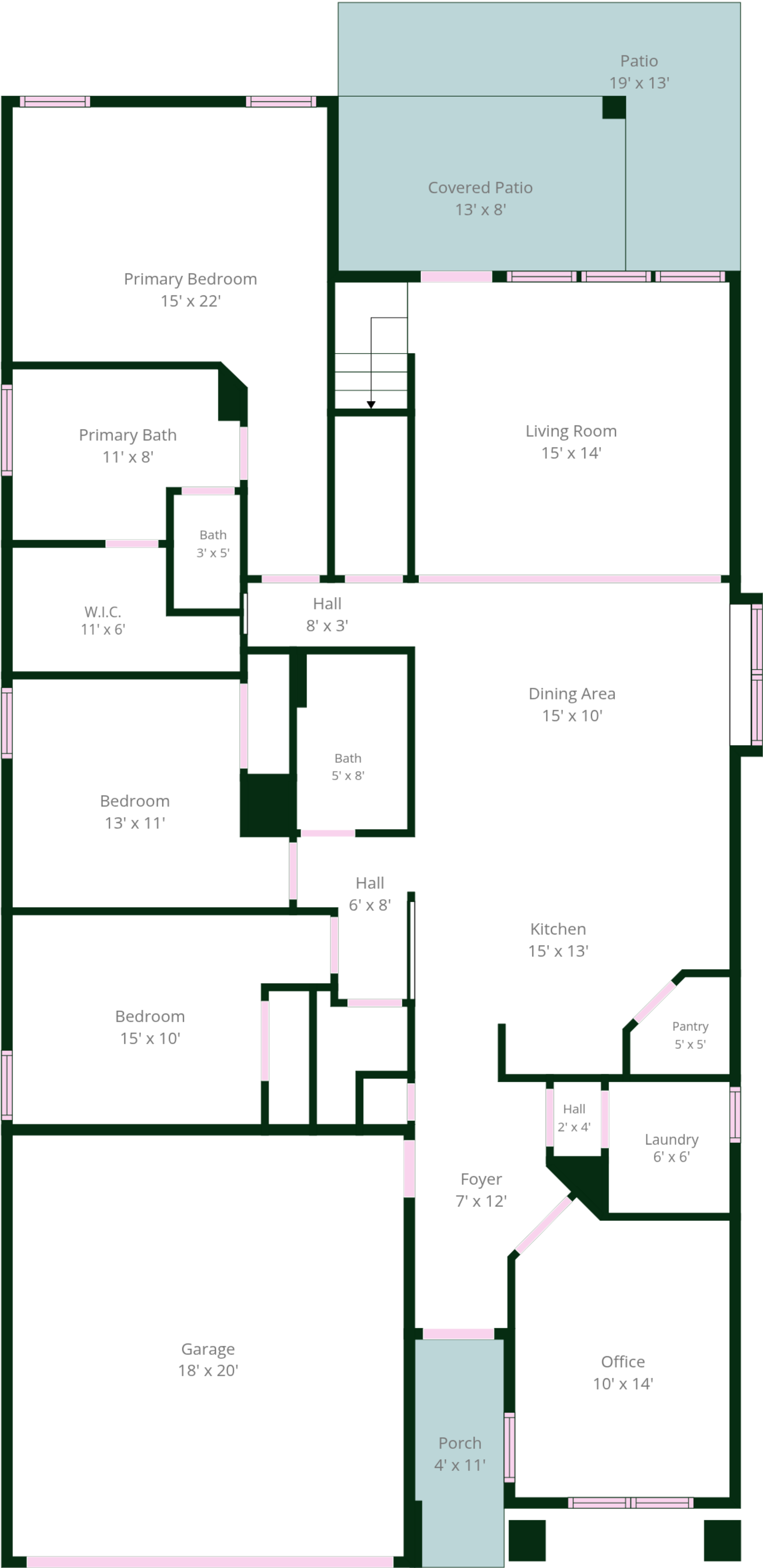
1st Floor
