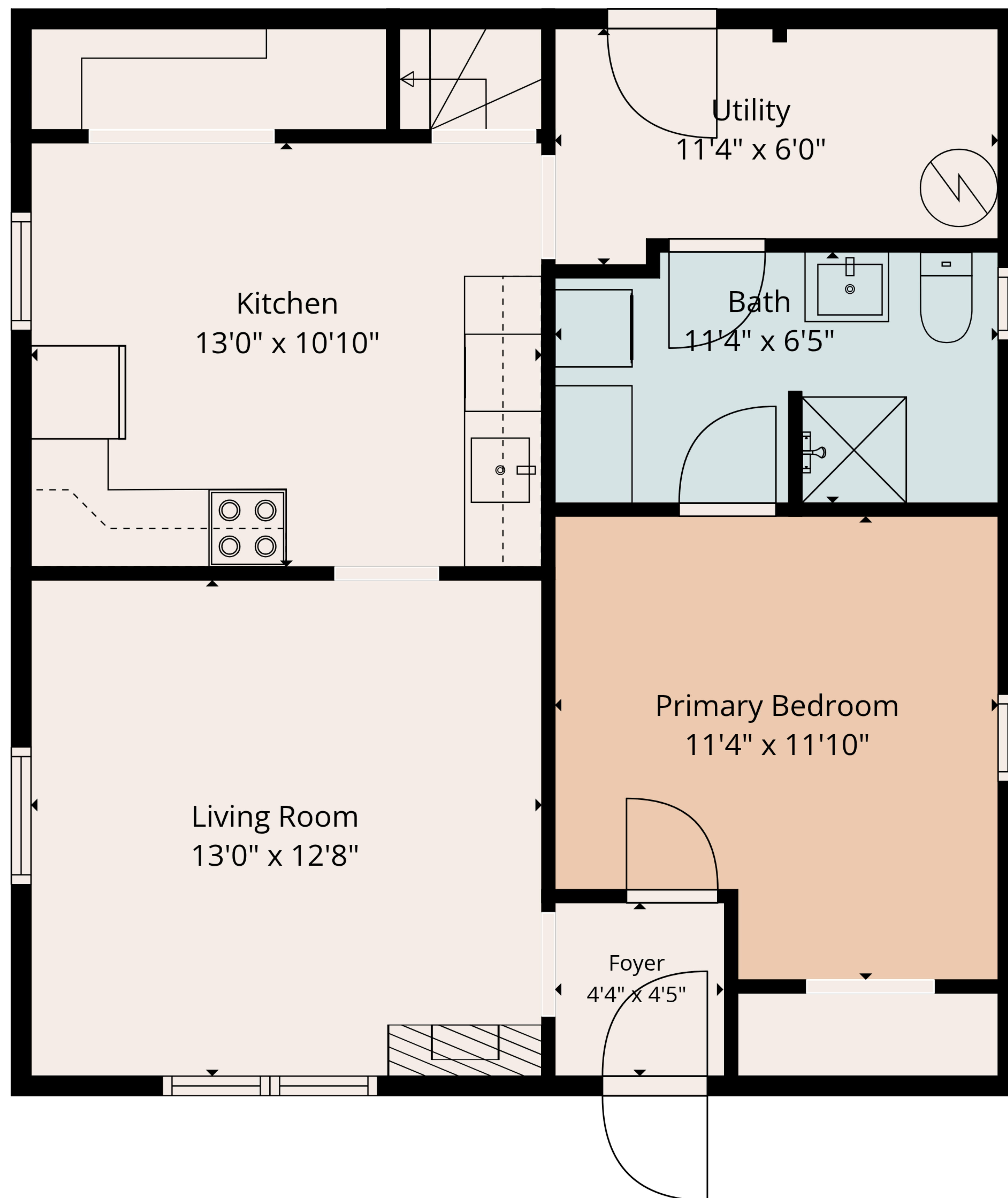
1st Floor
