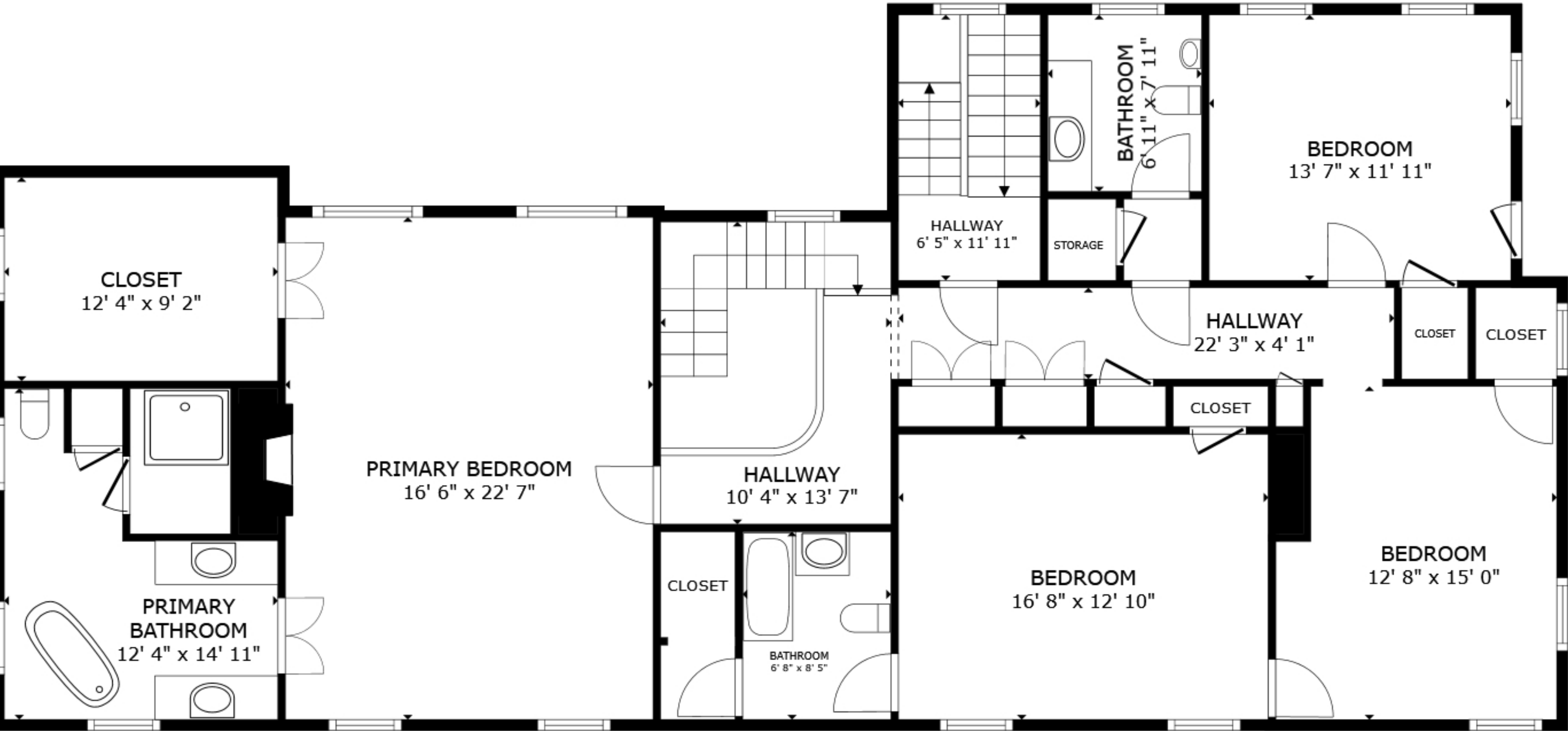
FLOOR 2
