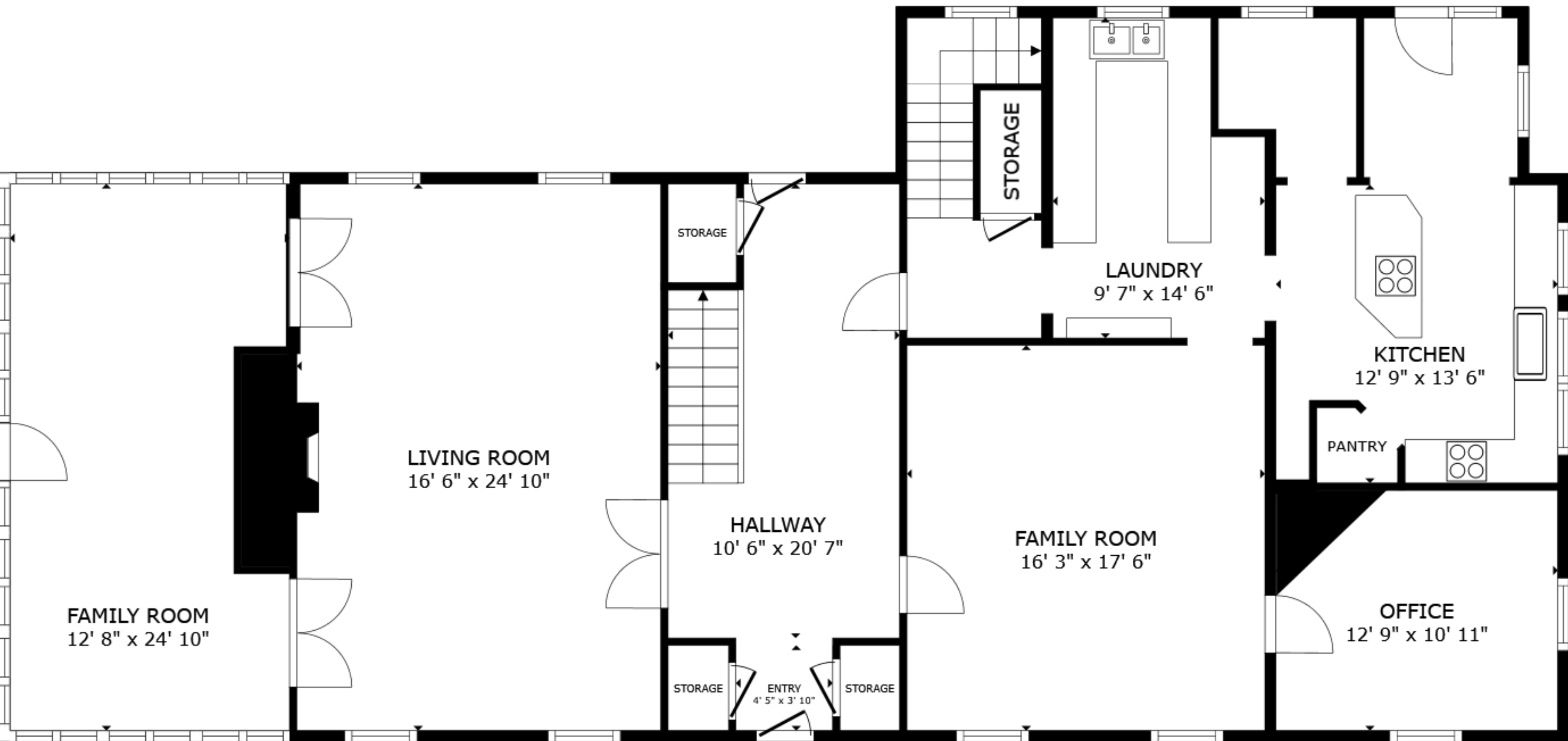
FLOOR 1
