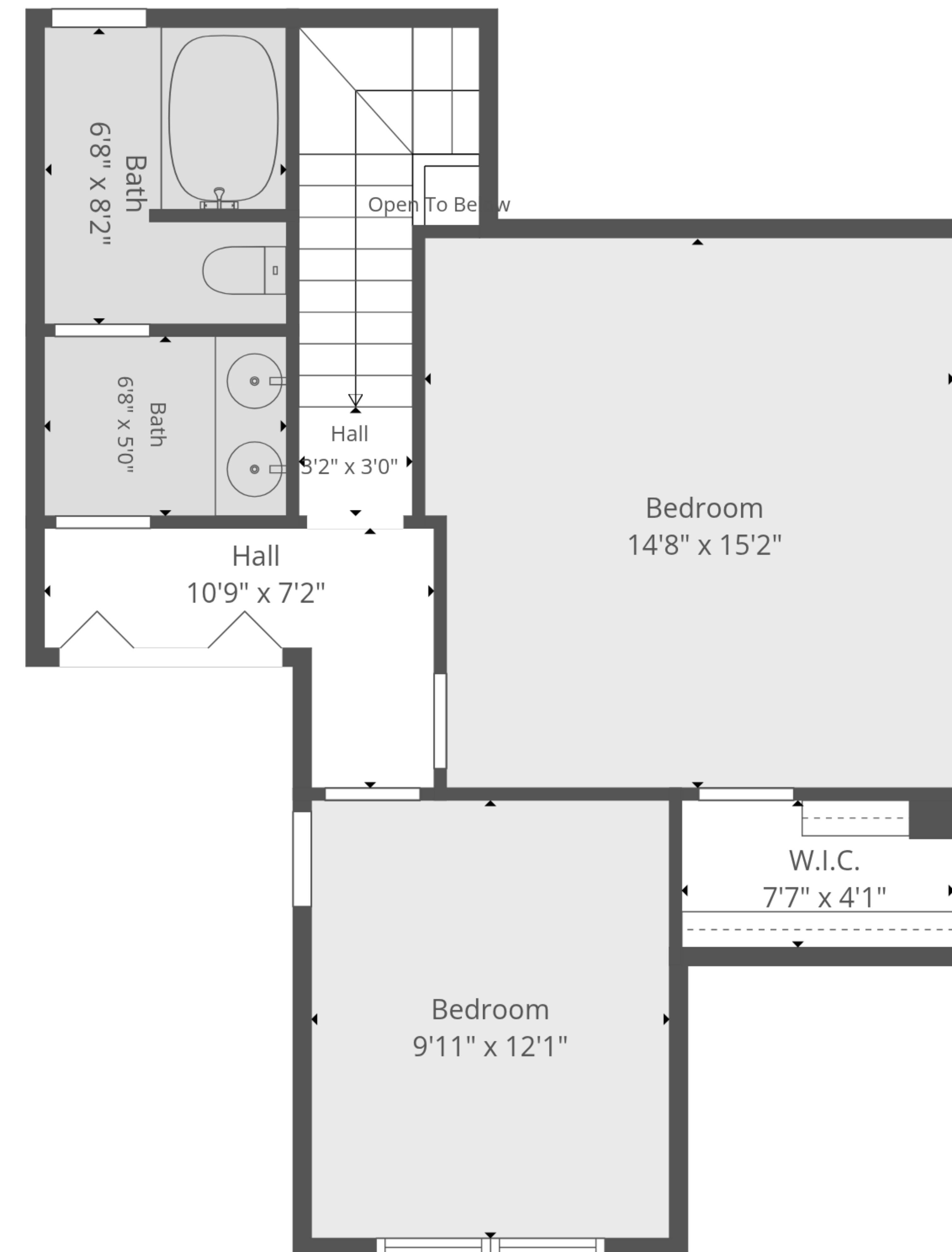
2nd Floor
