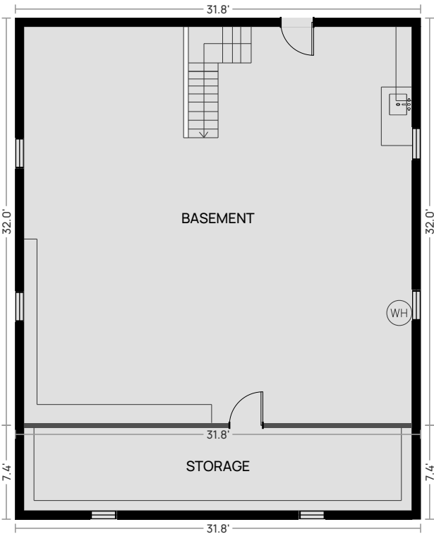
BASEMENT Below grade · 7'6" ceiling · No finished area
