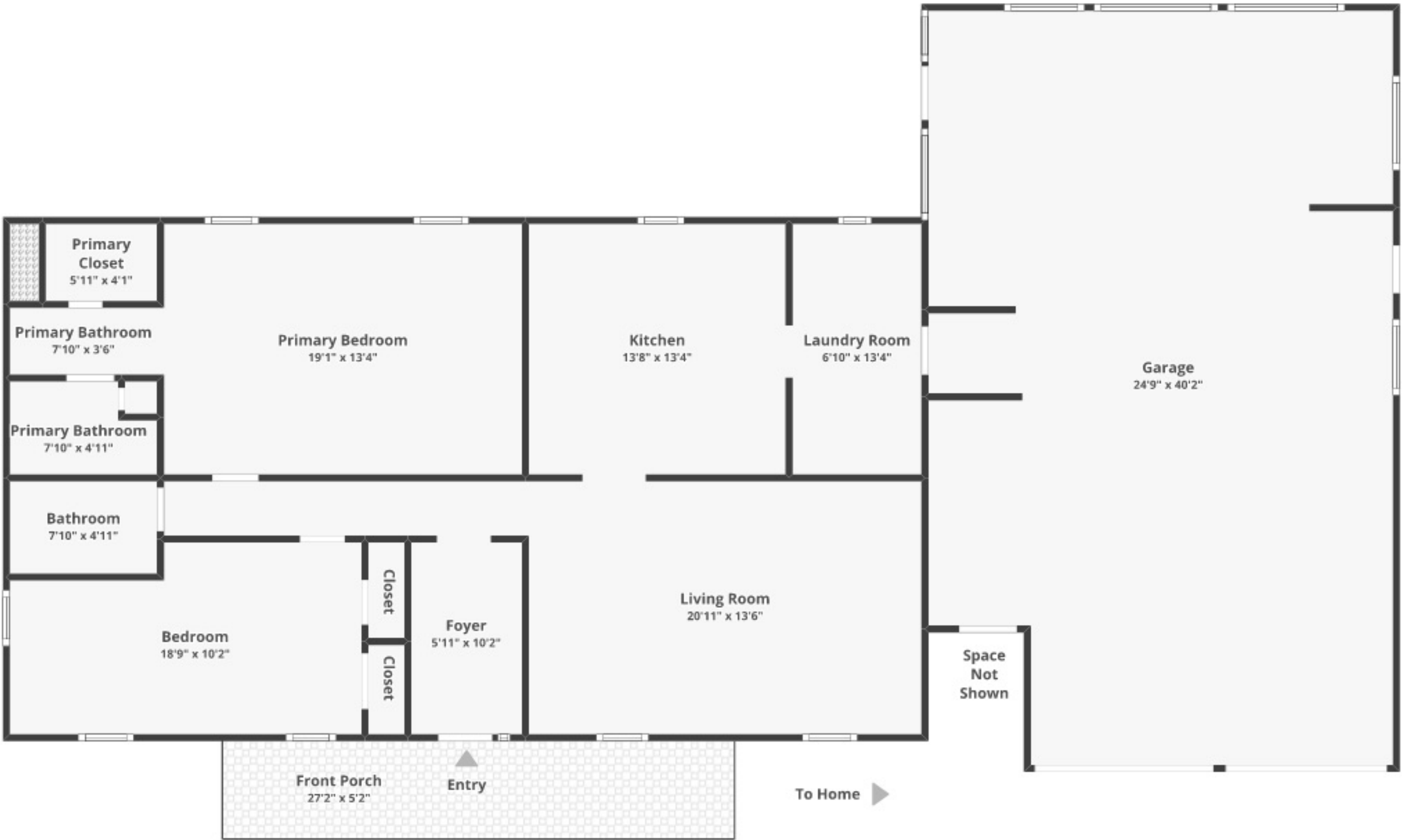
FLOOR 1
