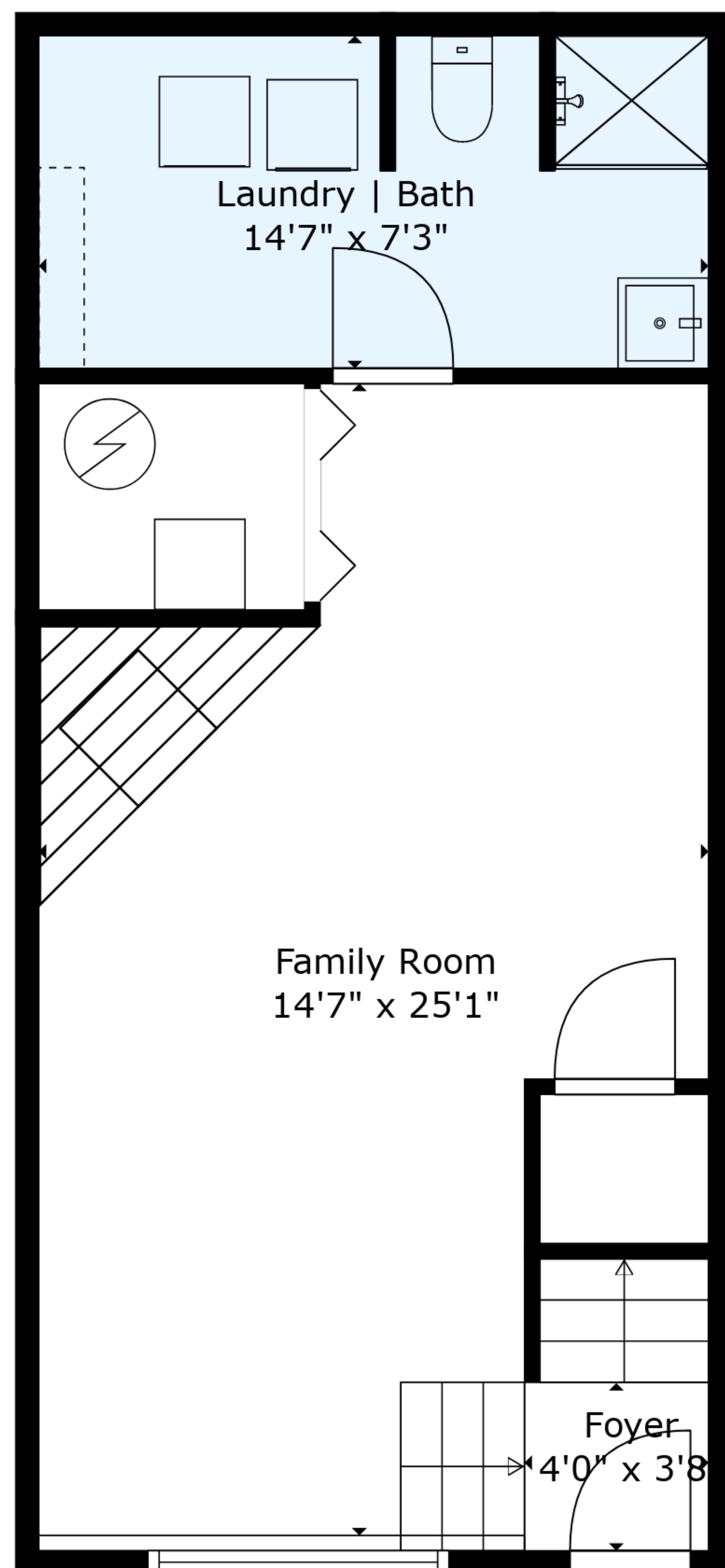
Floor 1
