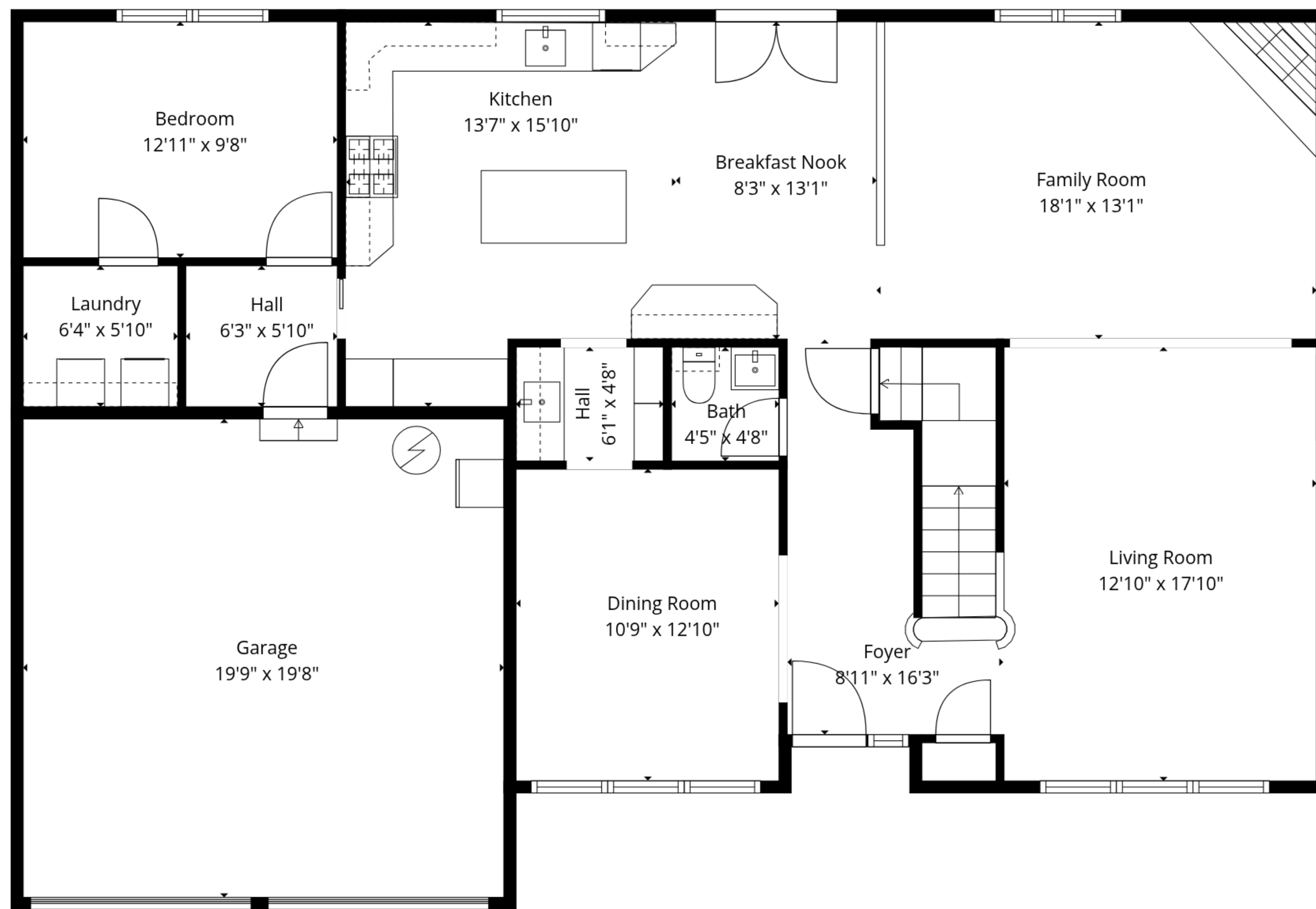
1st Floor
