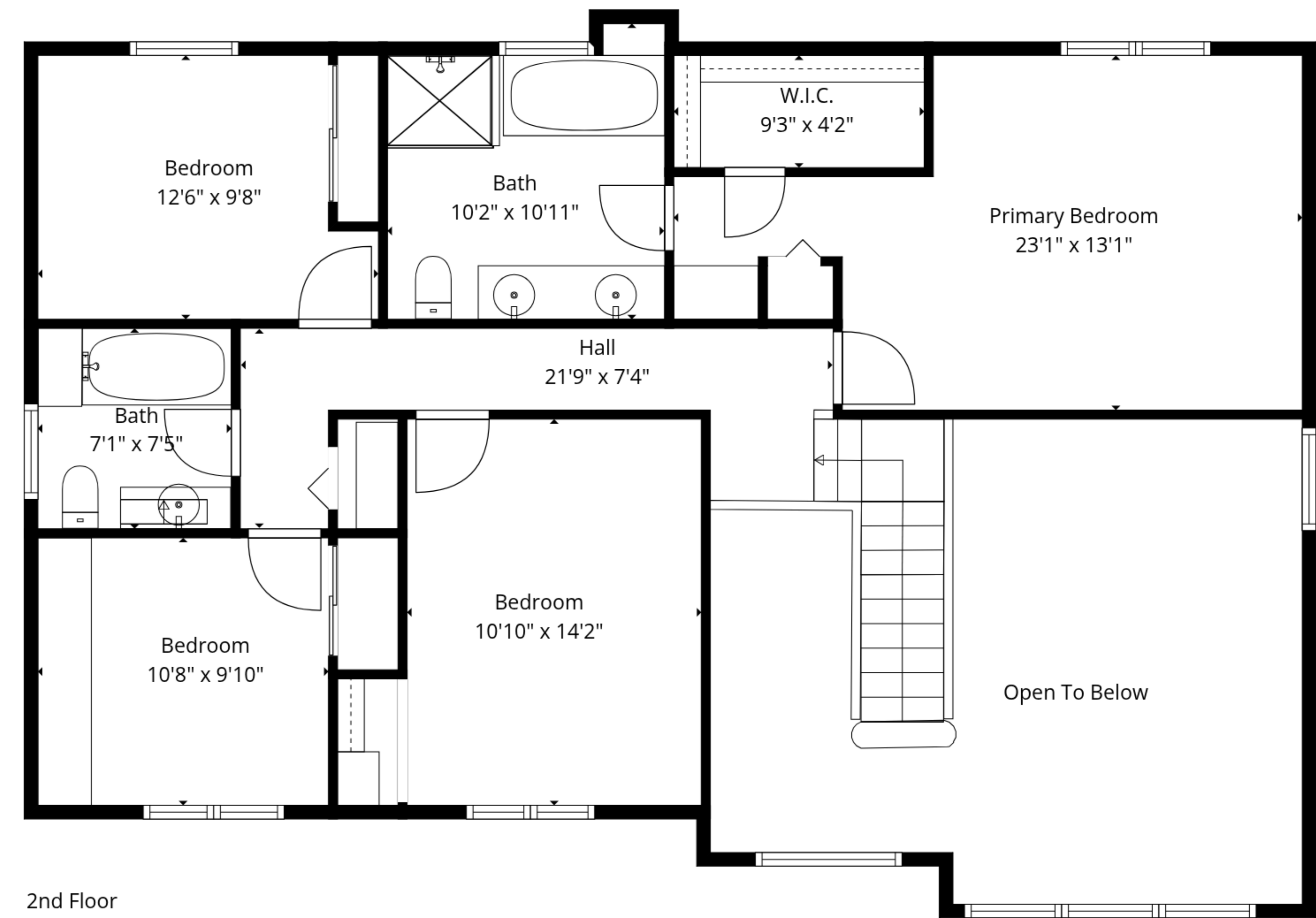
2nd Floor
