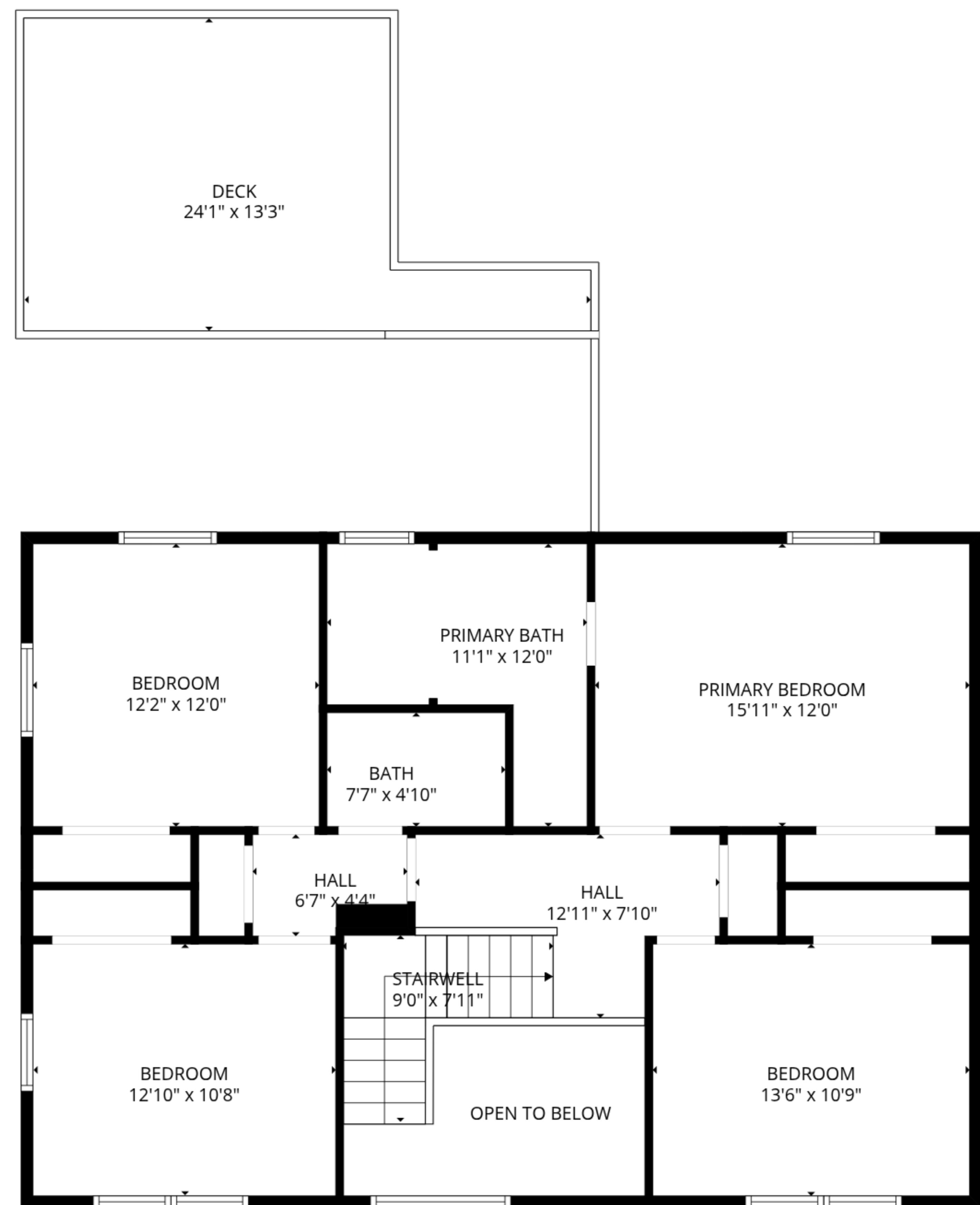
2nd floor
