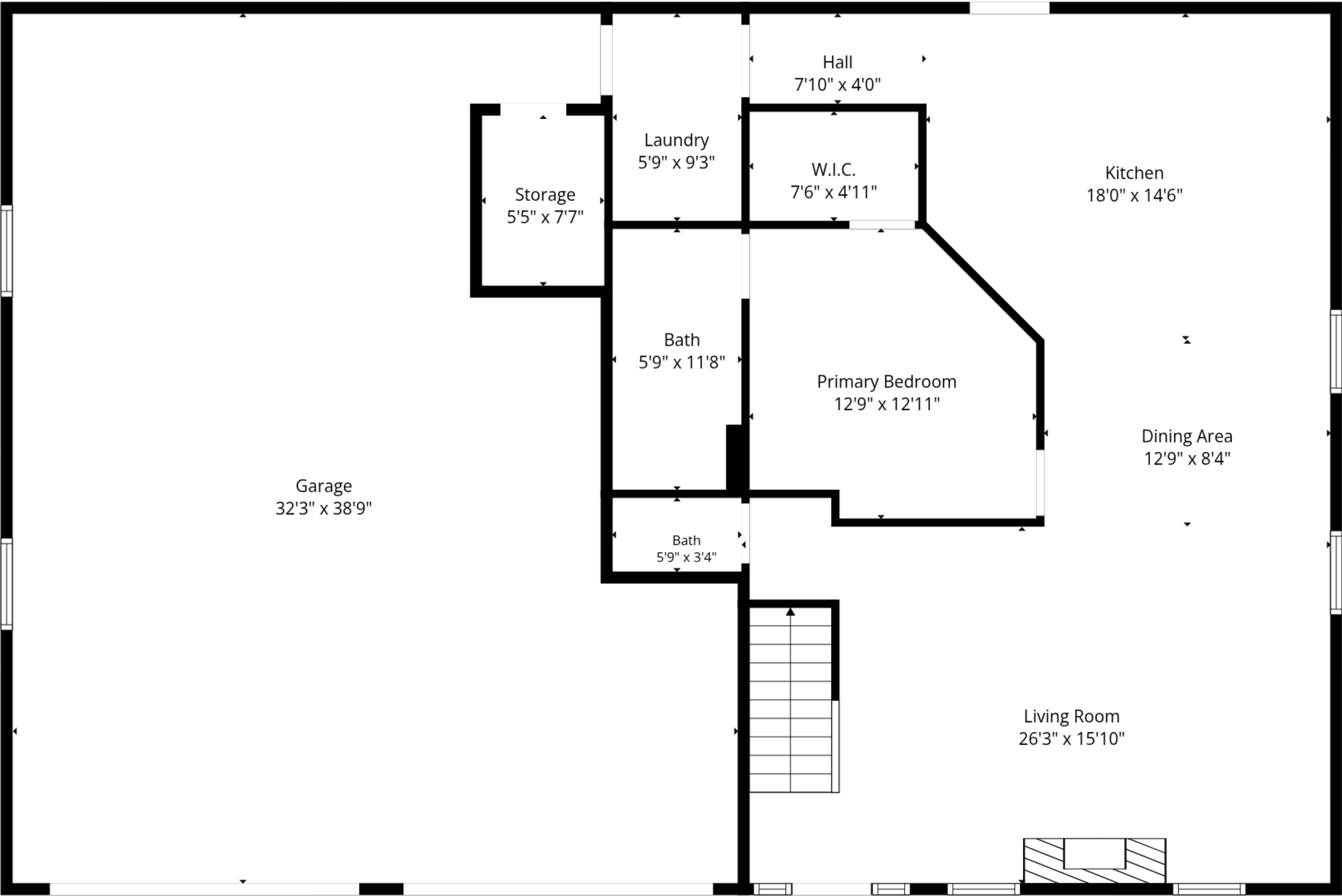
1st Floor
