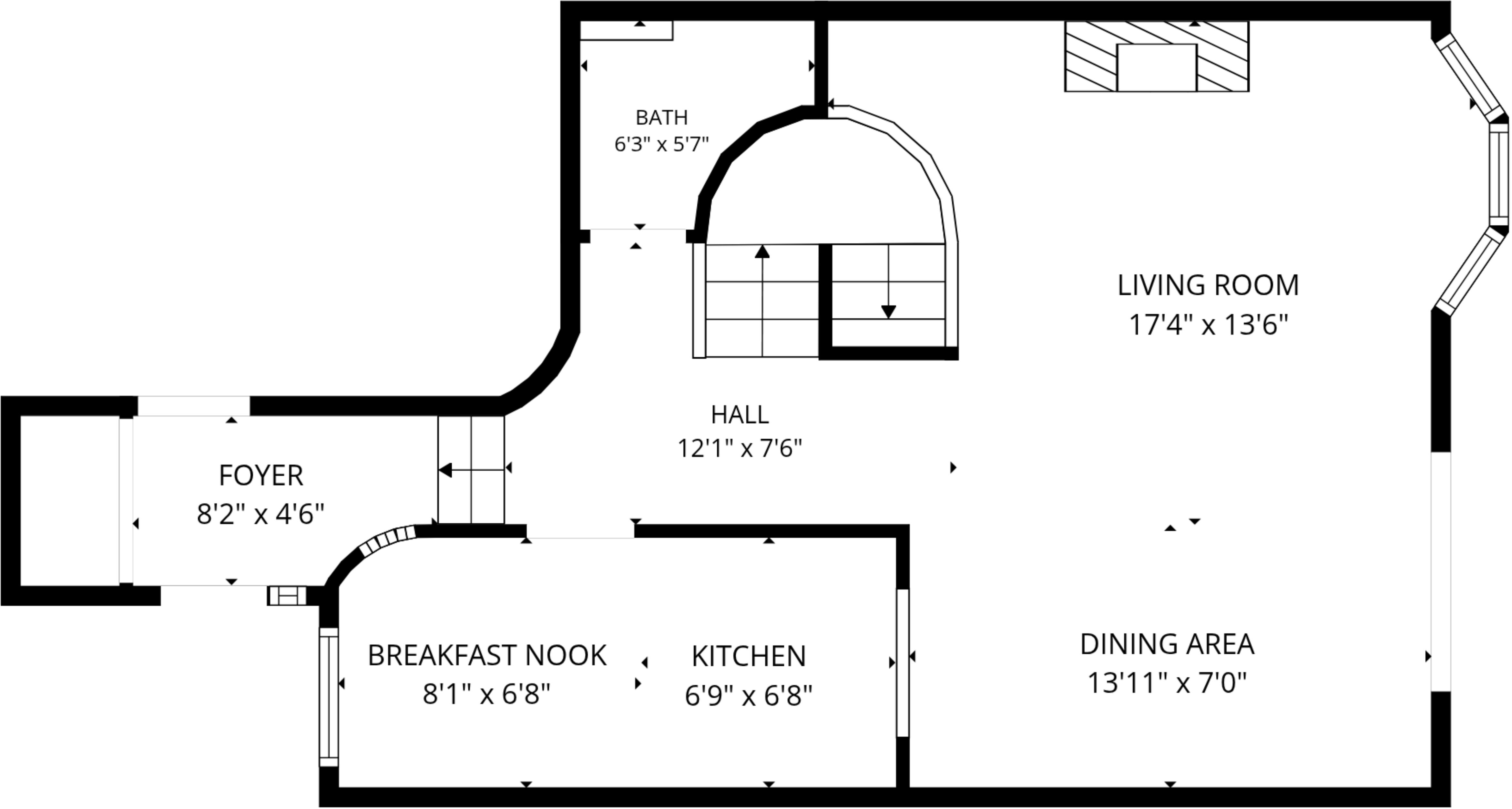
2nd floor
