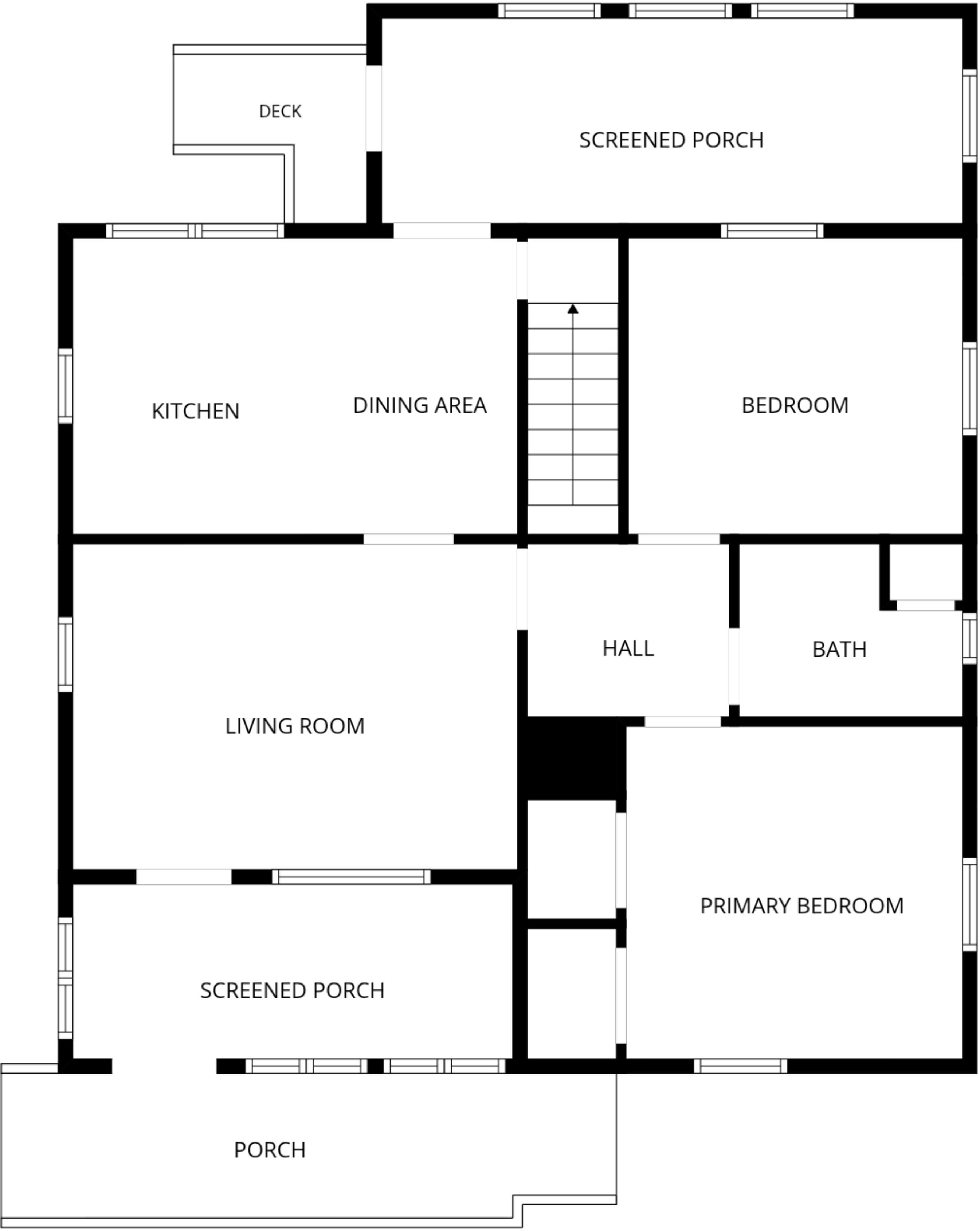
2nd floor
