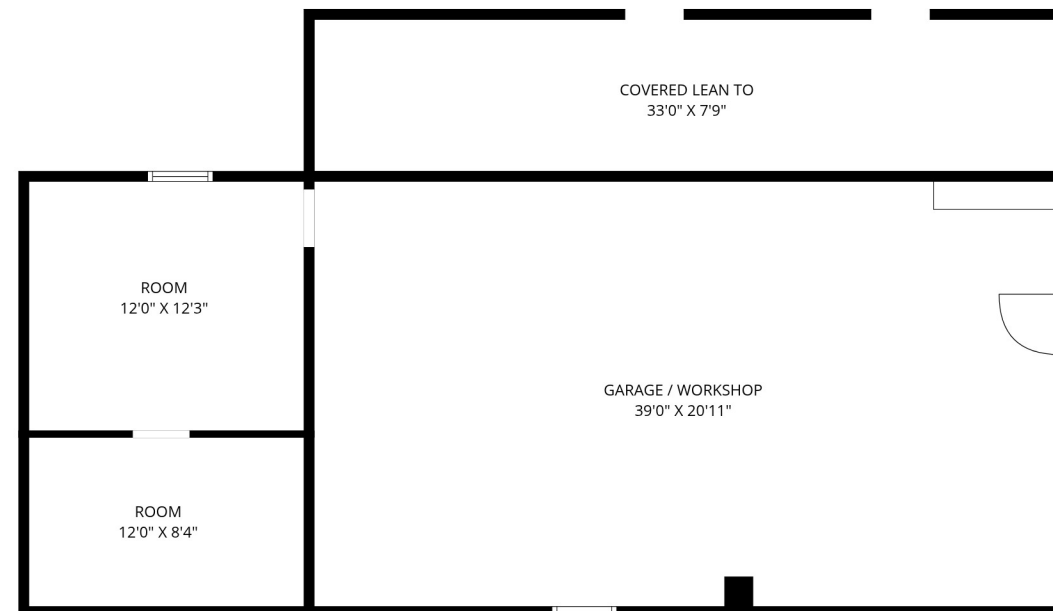
DETACHED GARAGE
