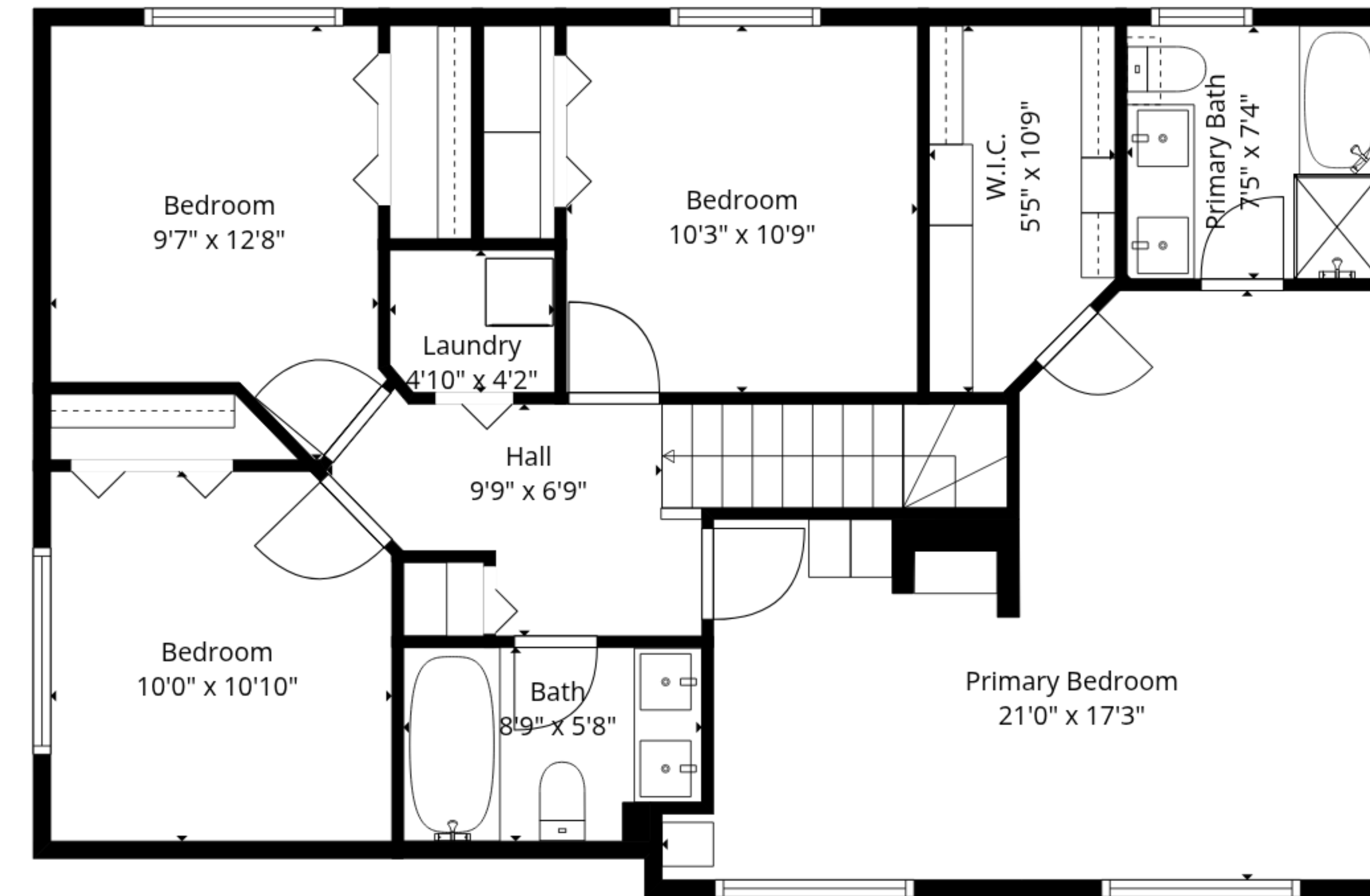
2nd Floor
