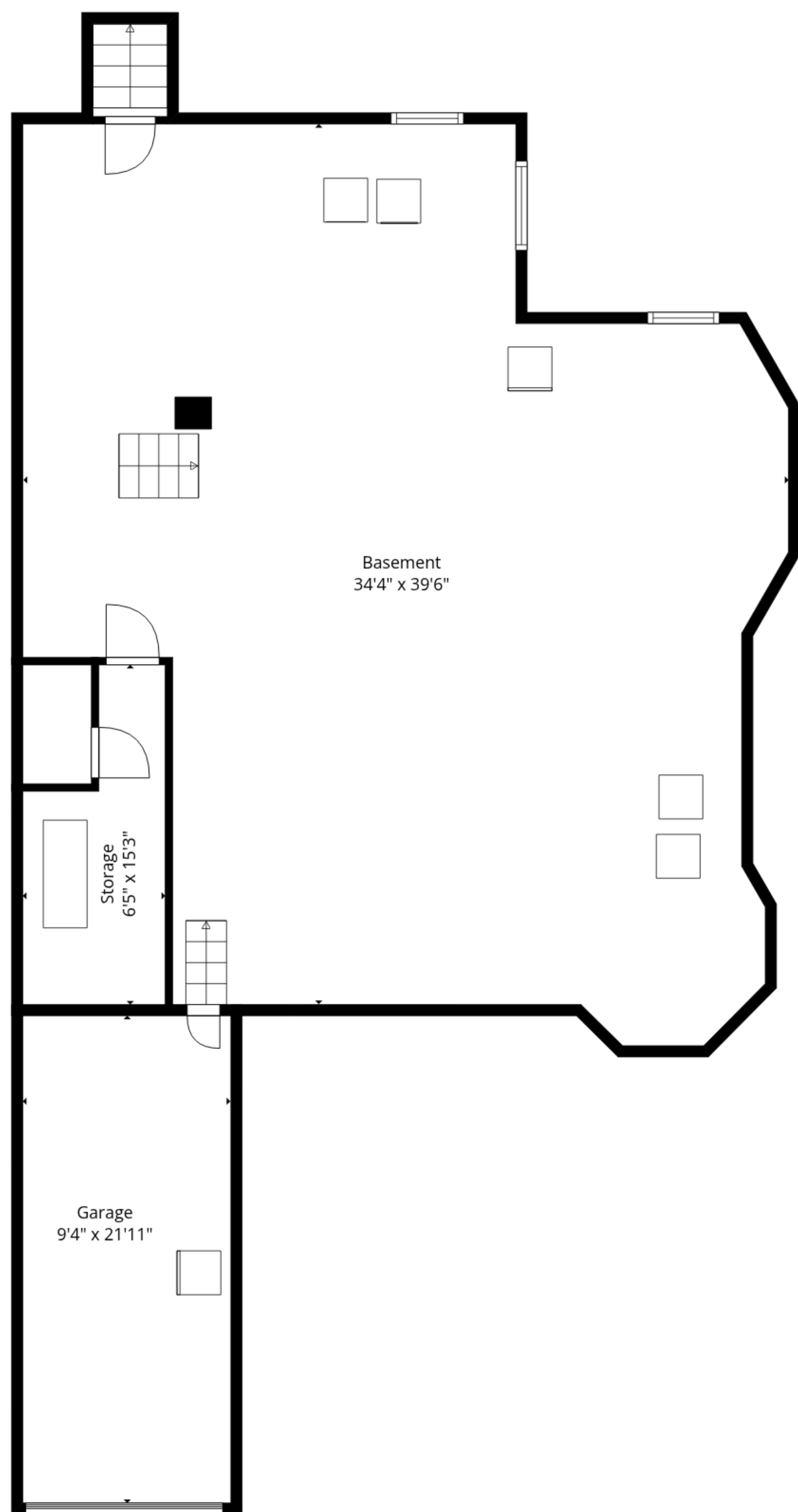
Basement
