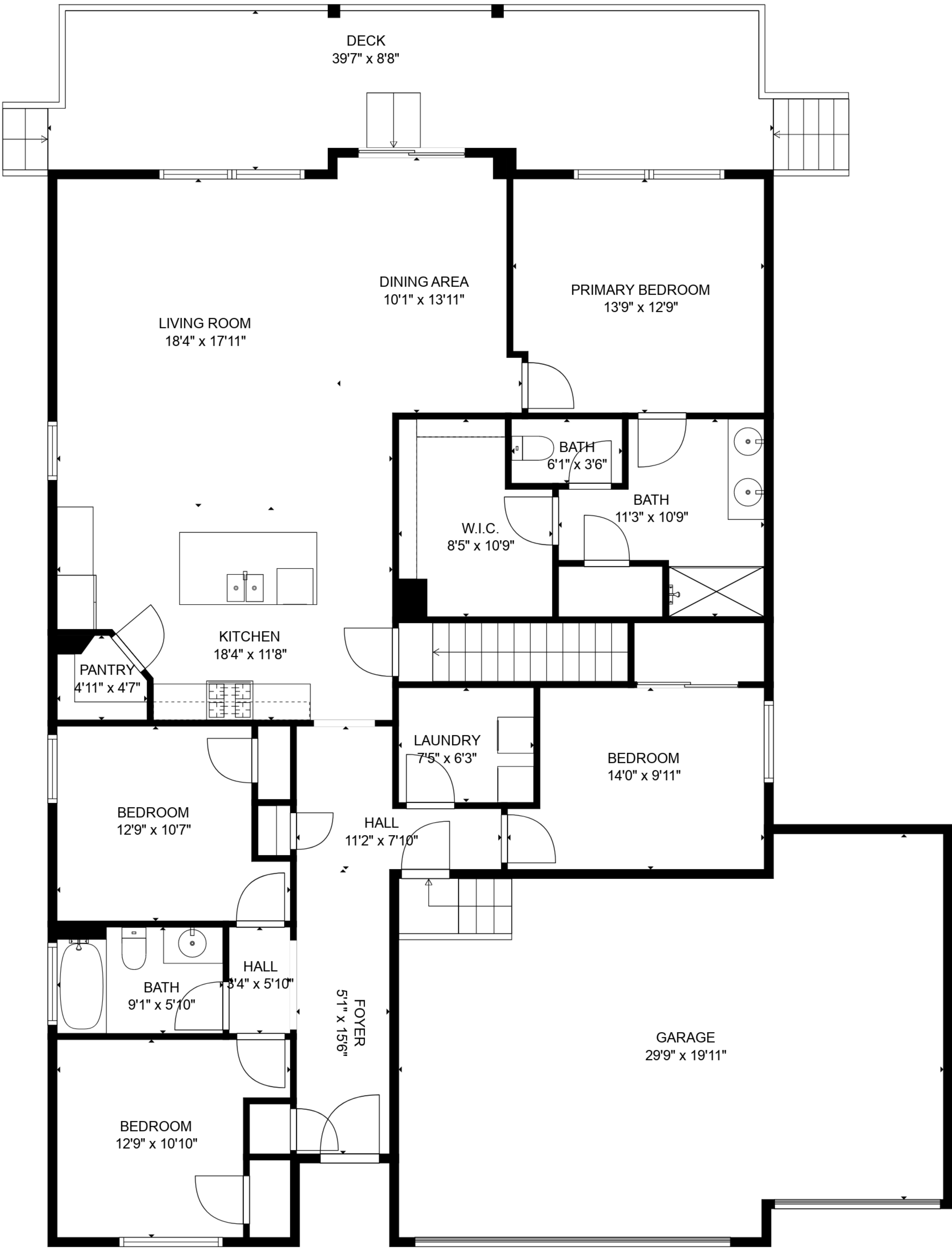
FLOOR 2
