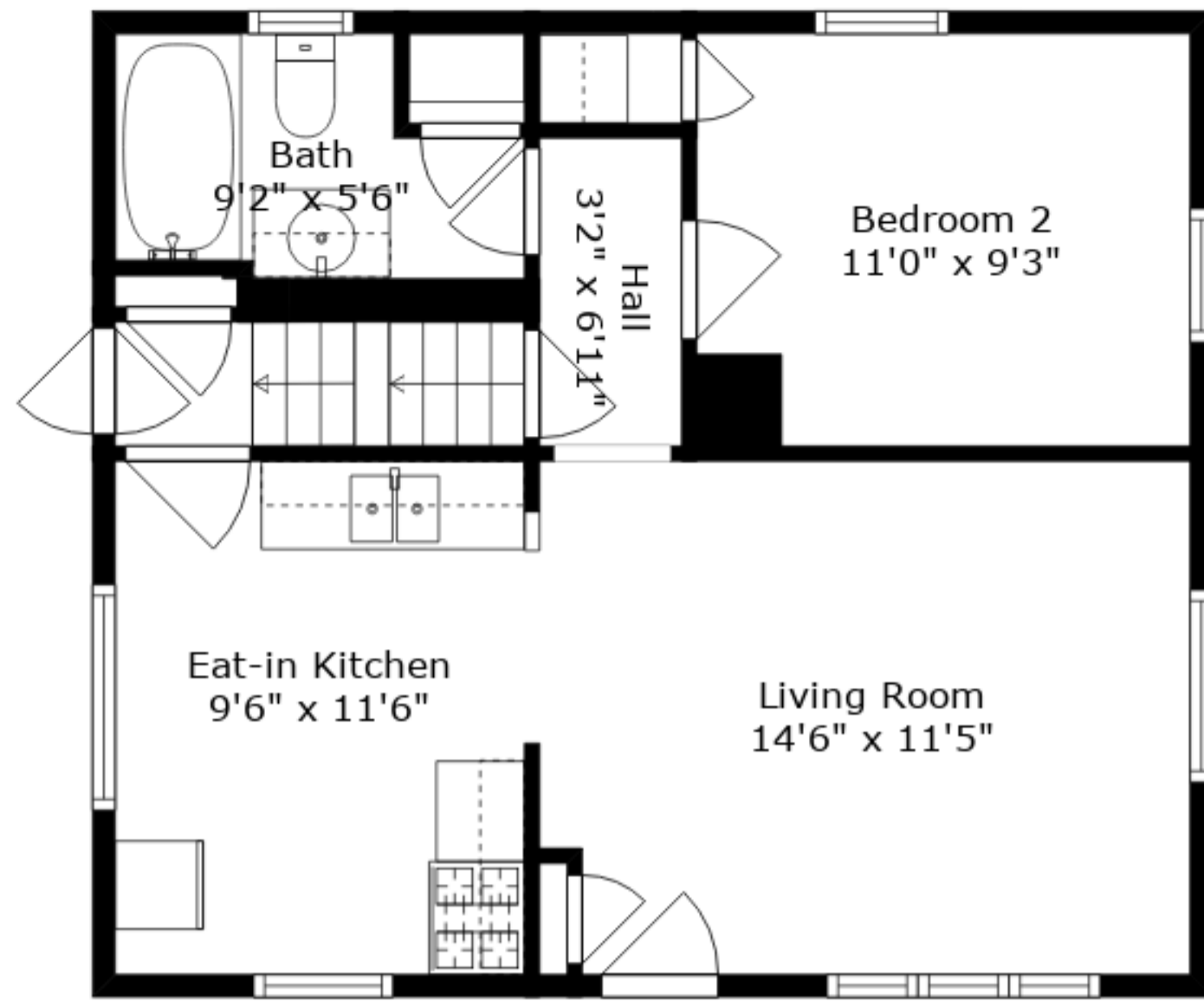
Main Floor
