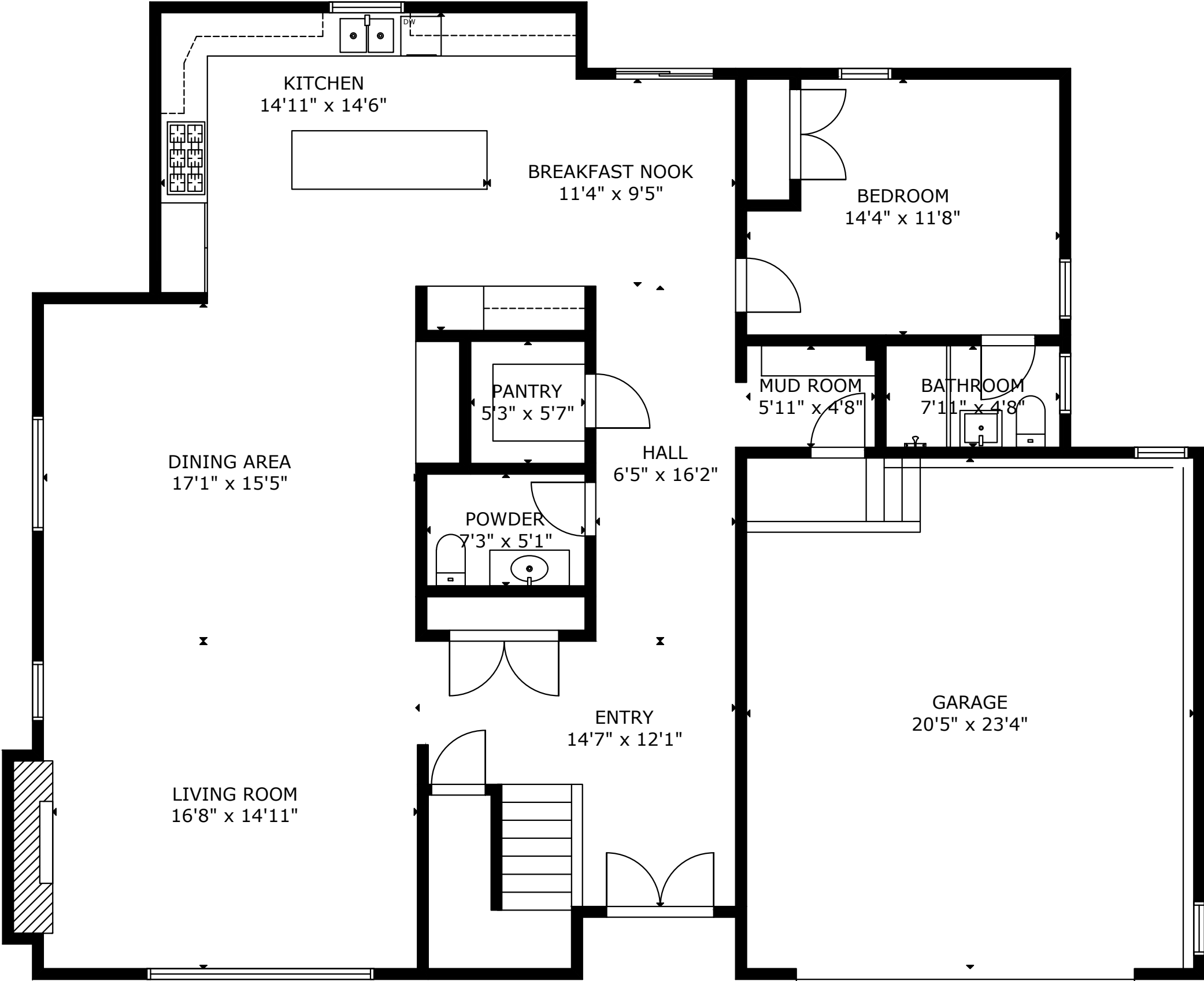
FIRST FLOOR
