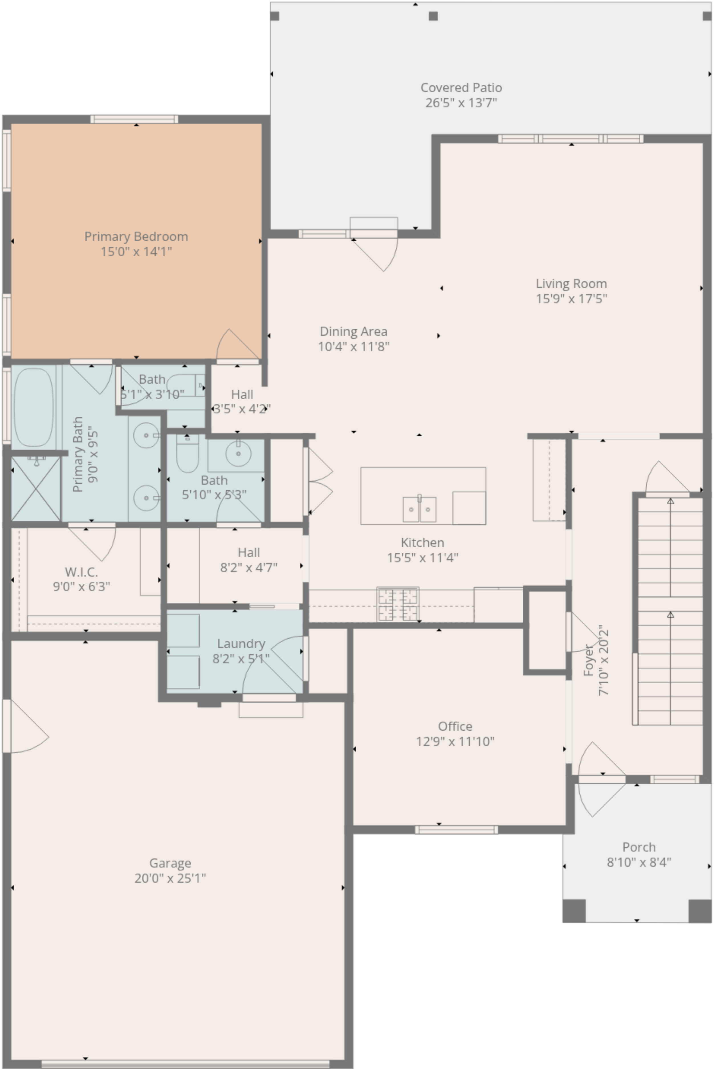
1st Floor
