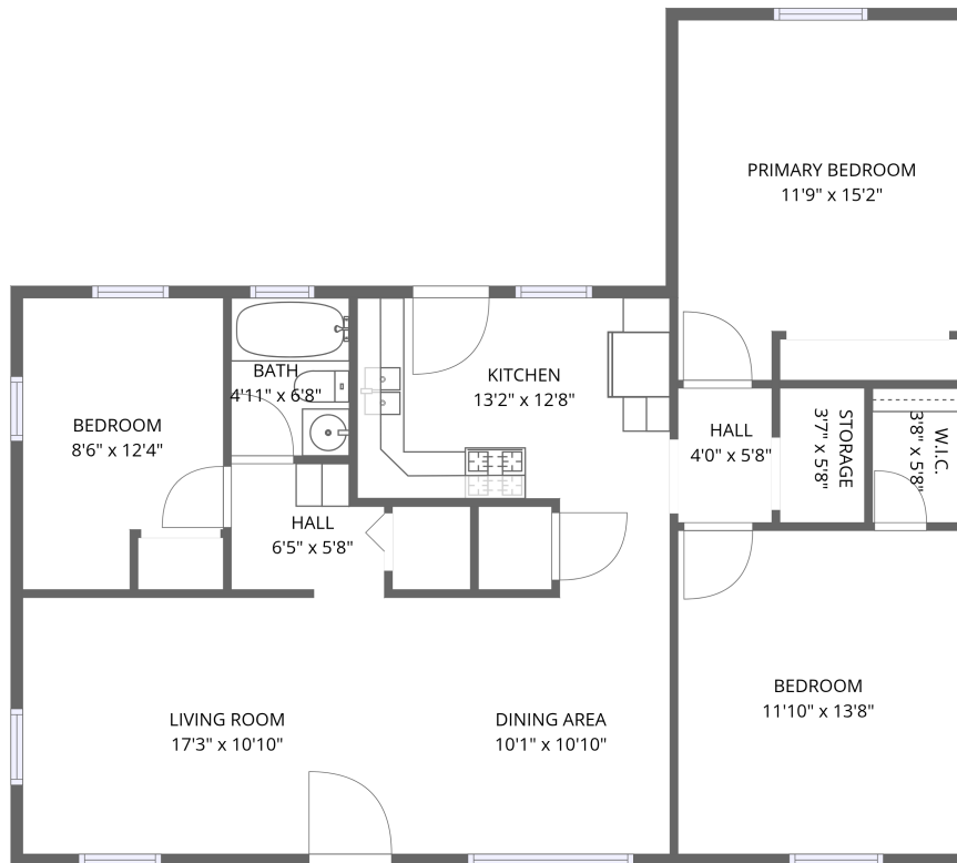
1st floor
