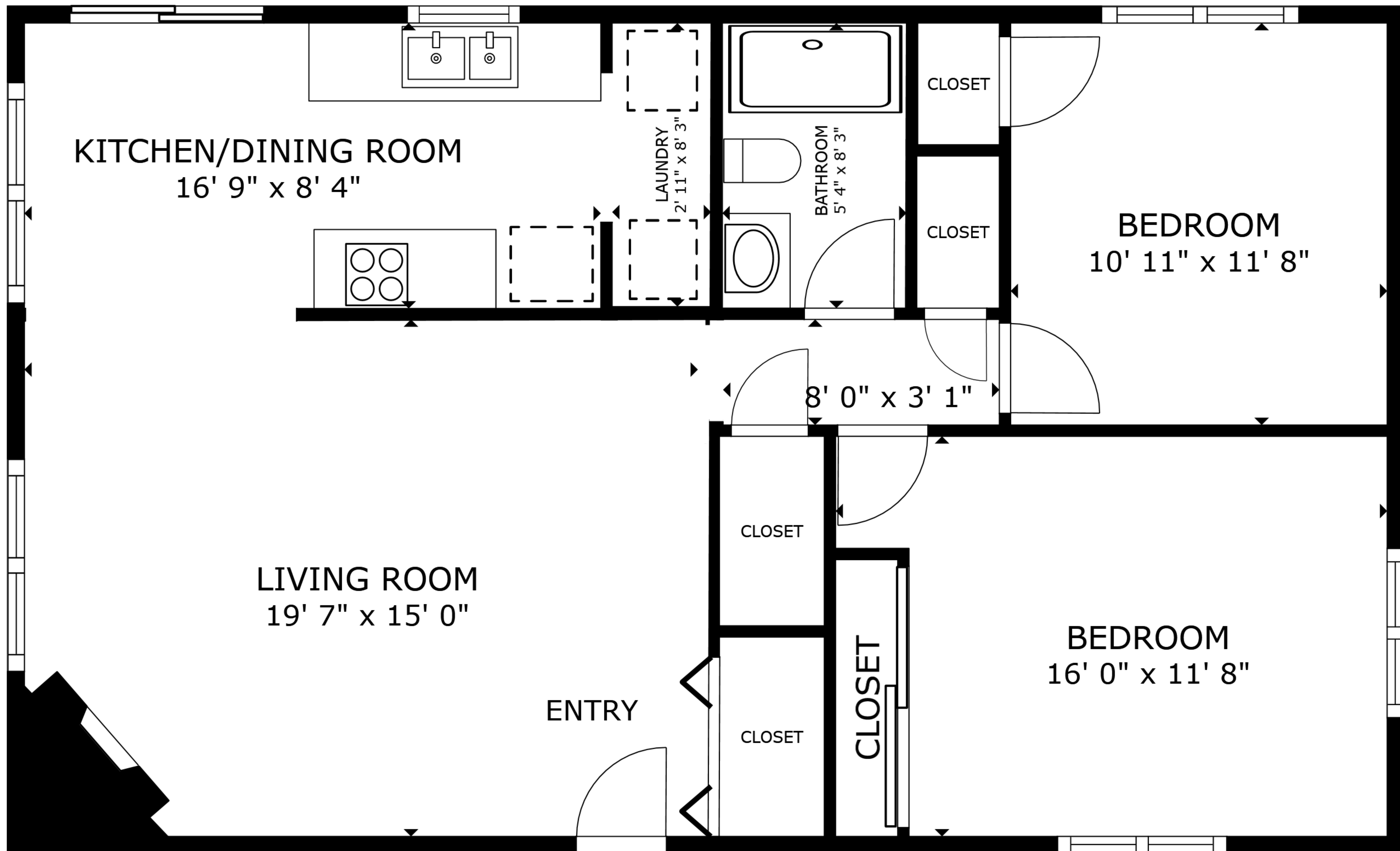
FLOOR PLAN
