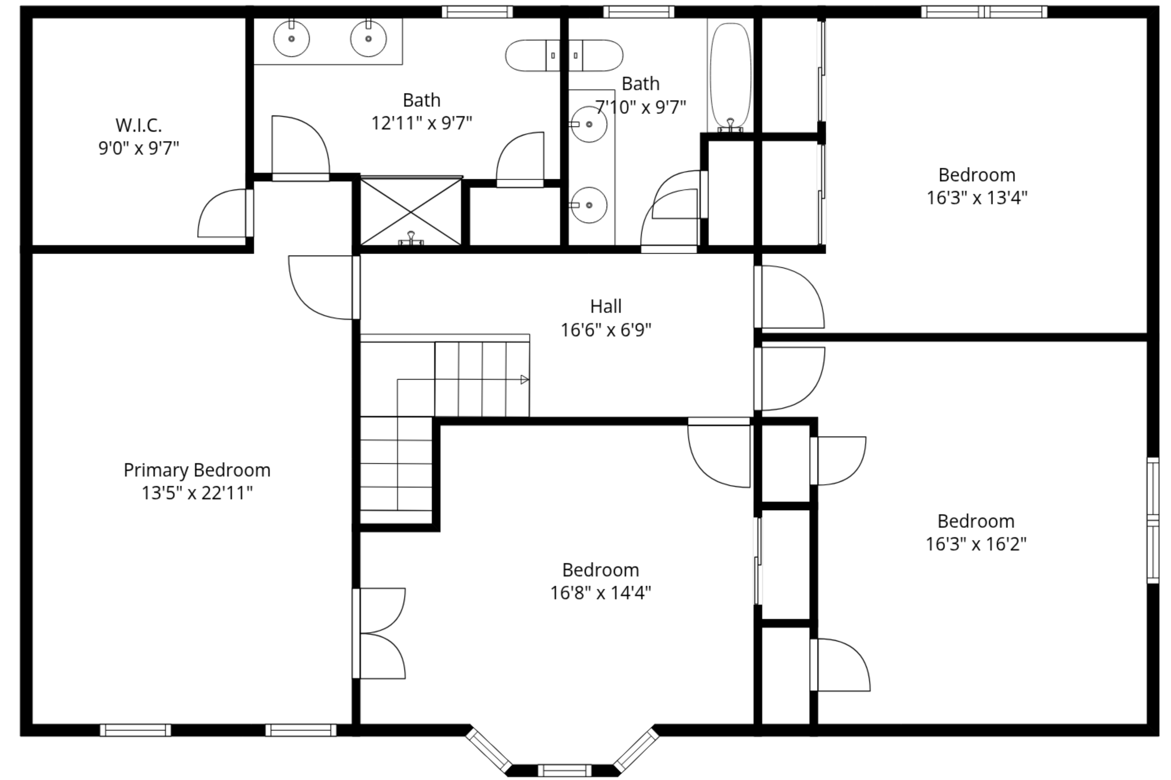
2nd Floor
