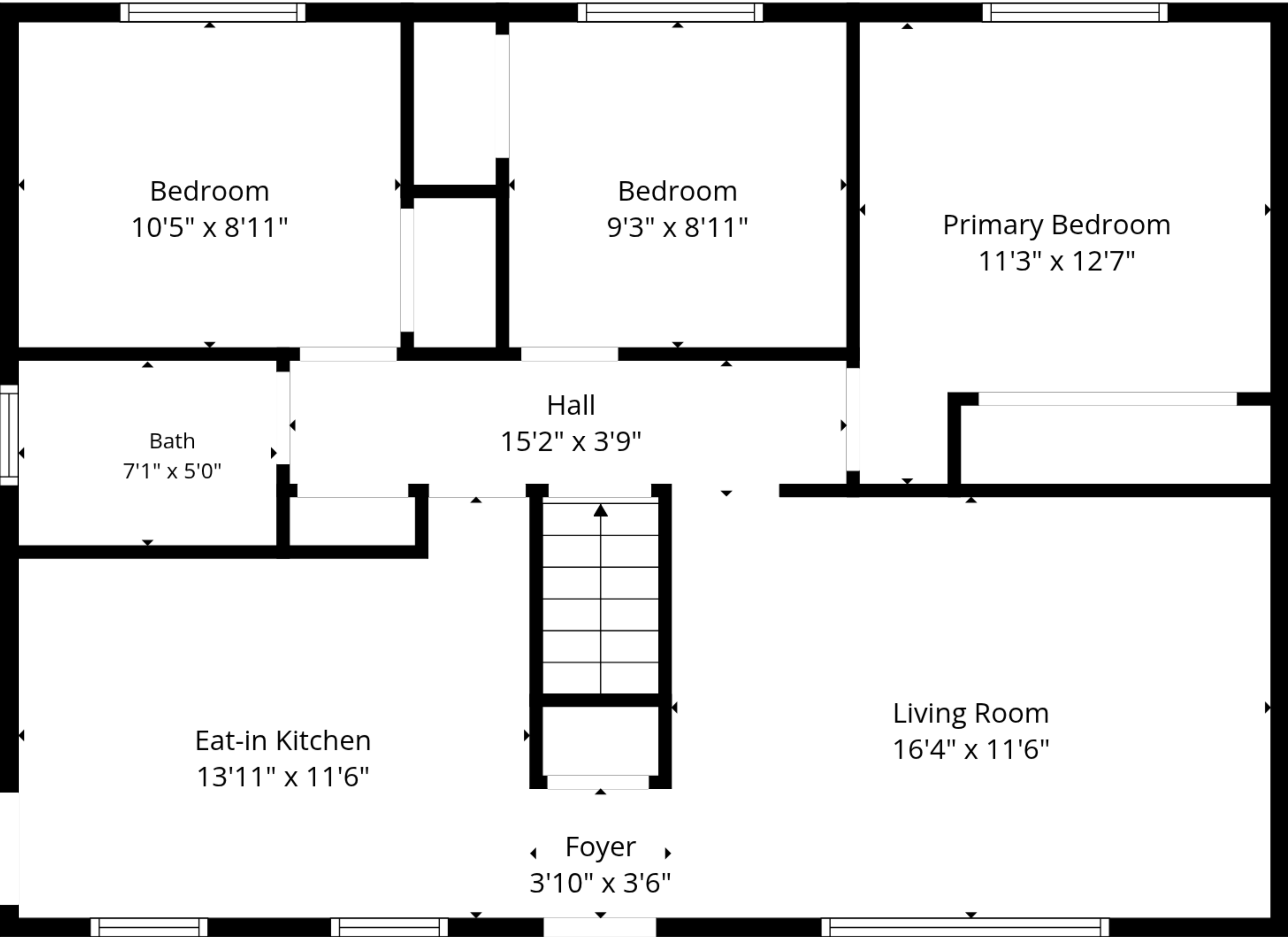
1st Floor
