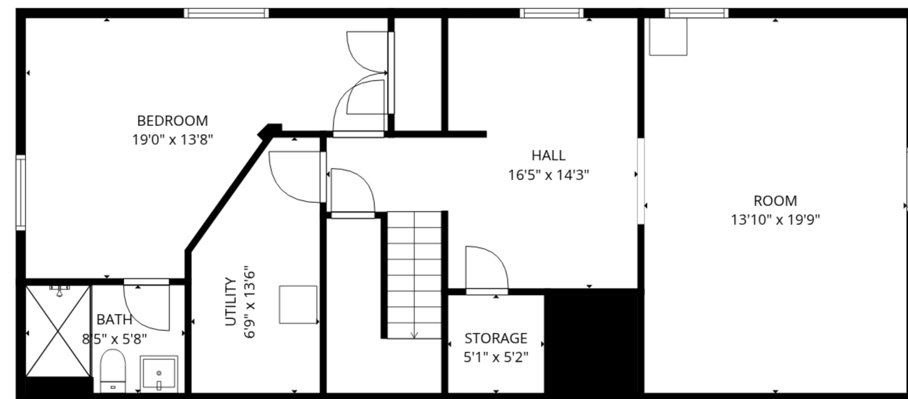
1st floor
