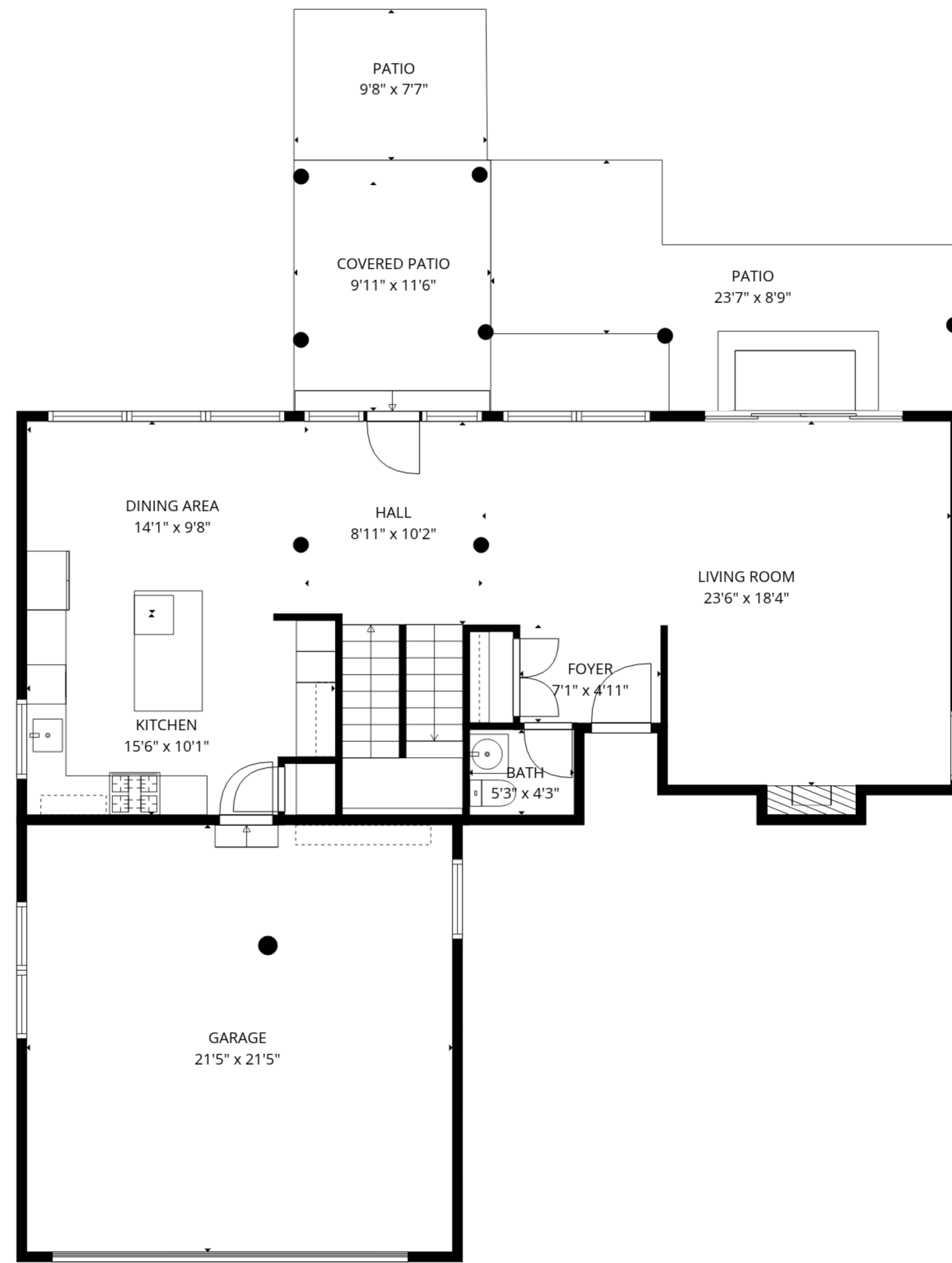
1st floor
