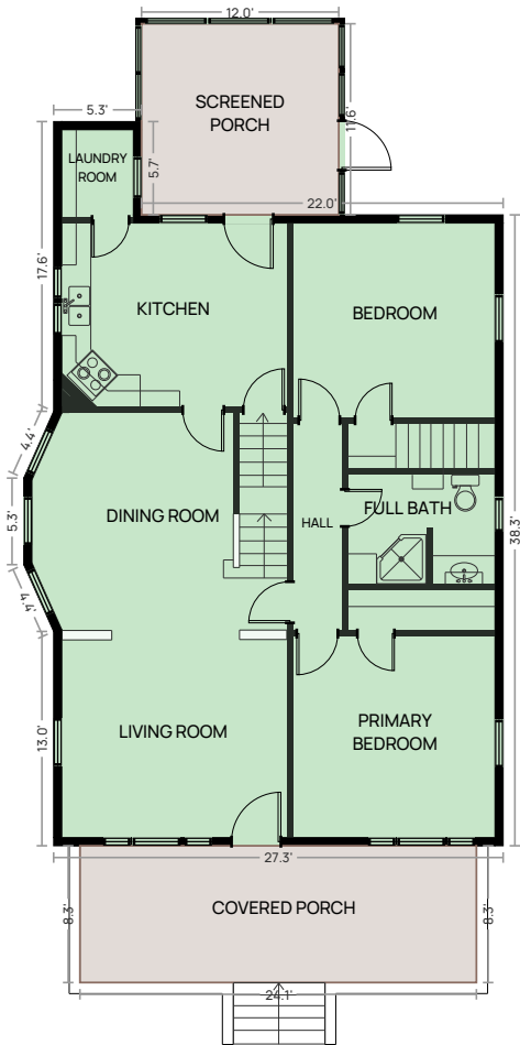
FIRST FLOOR Above grade - 9'1" ceiling - GLA 1,094 sq ft
