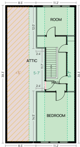
SECOND FLOOR Above grade - 7'5" ceiling GLA 401 sq ft
