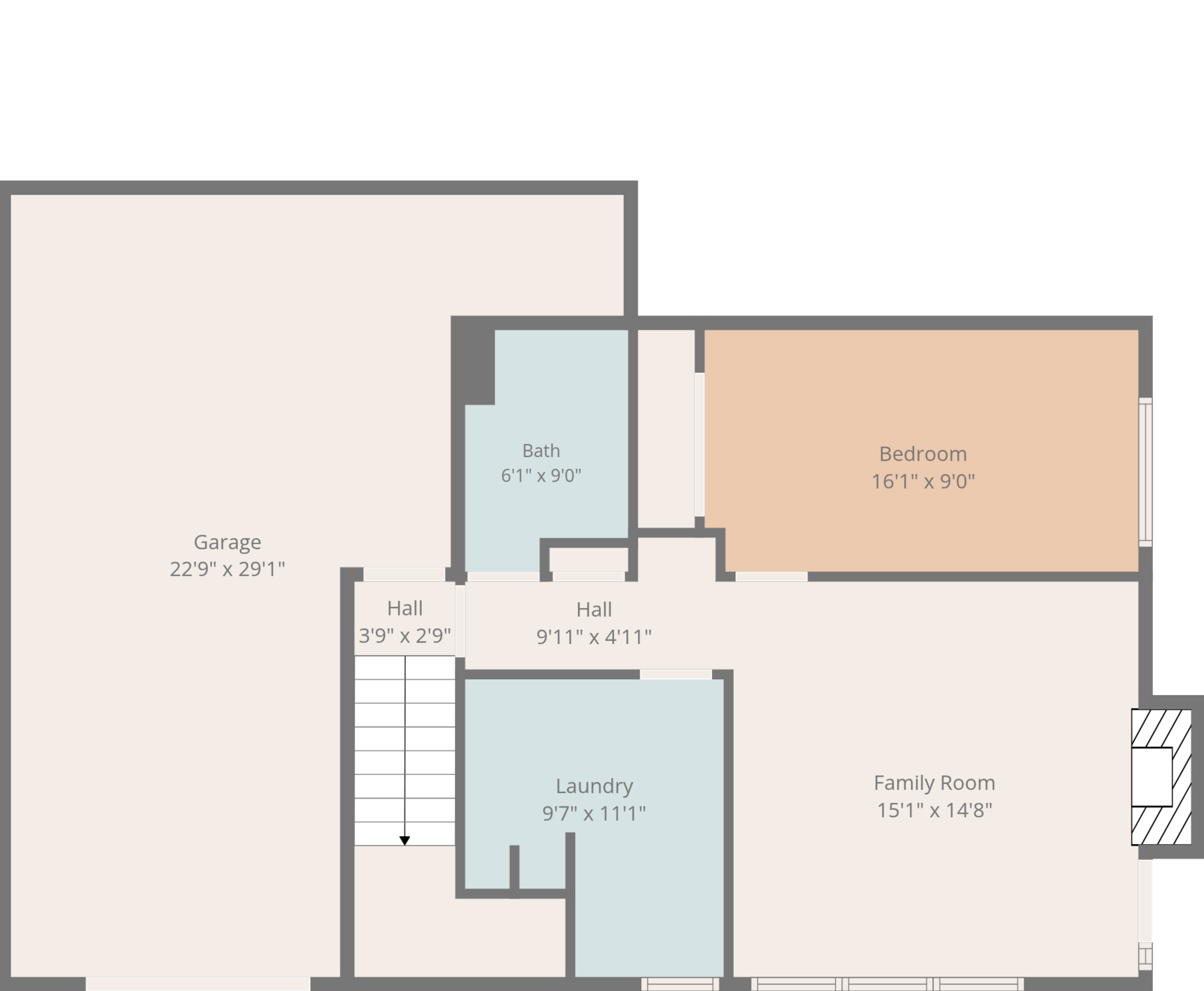
1st Floor
