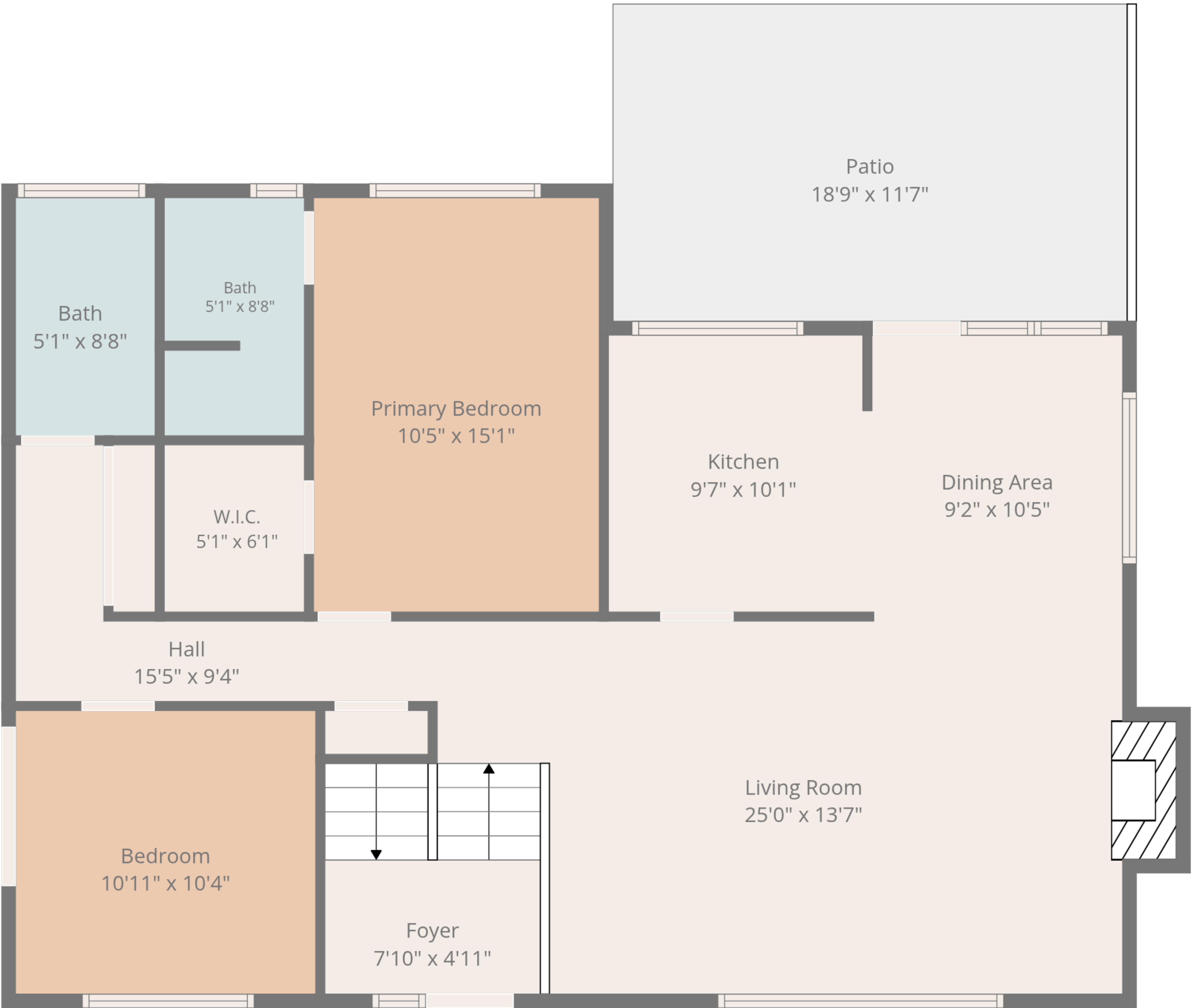
2nd Floor
