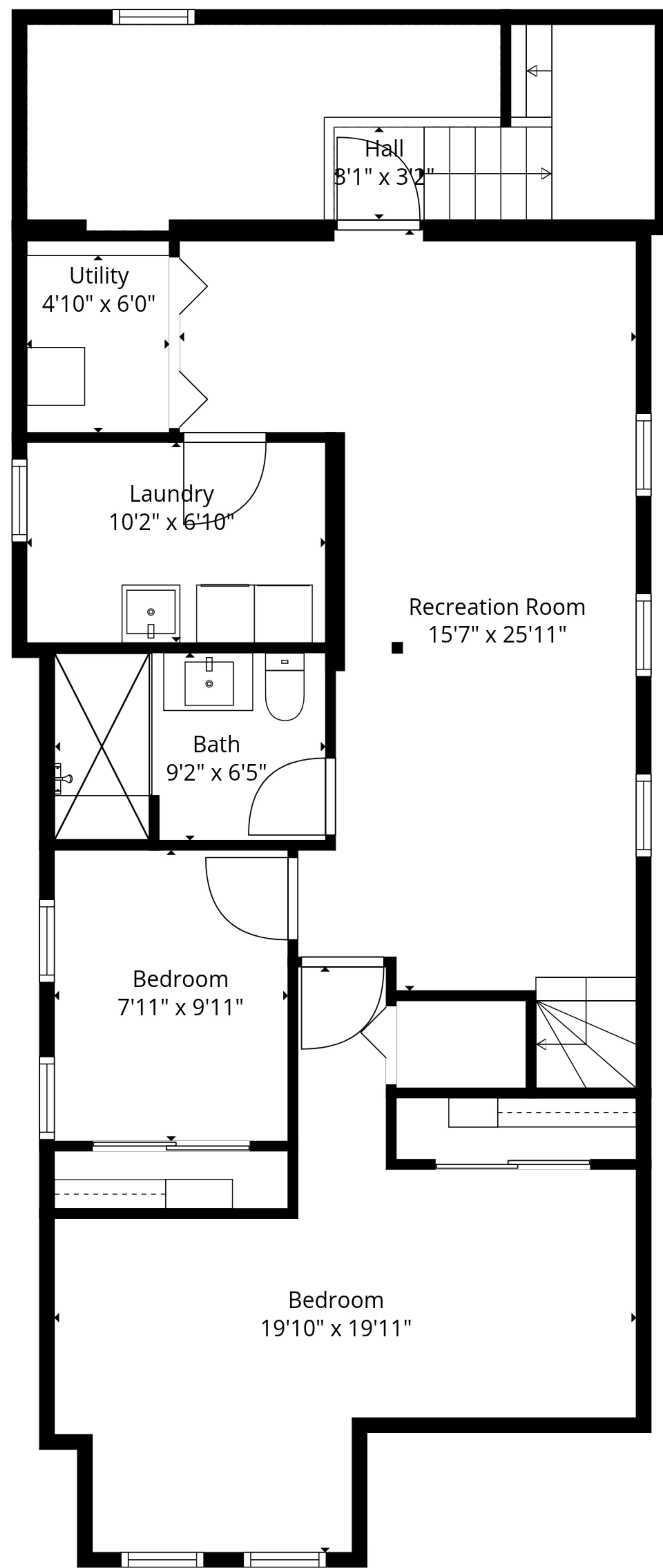
Basement 1
