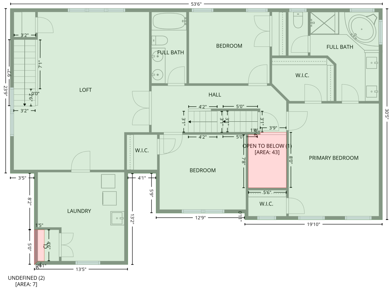
FLOOR 2 [AREA: 1605]
