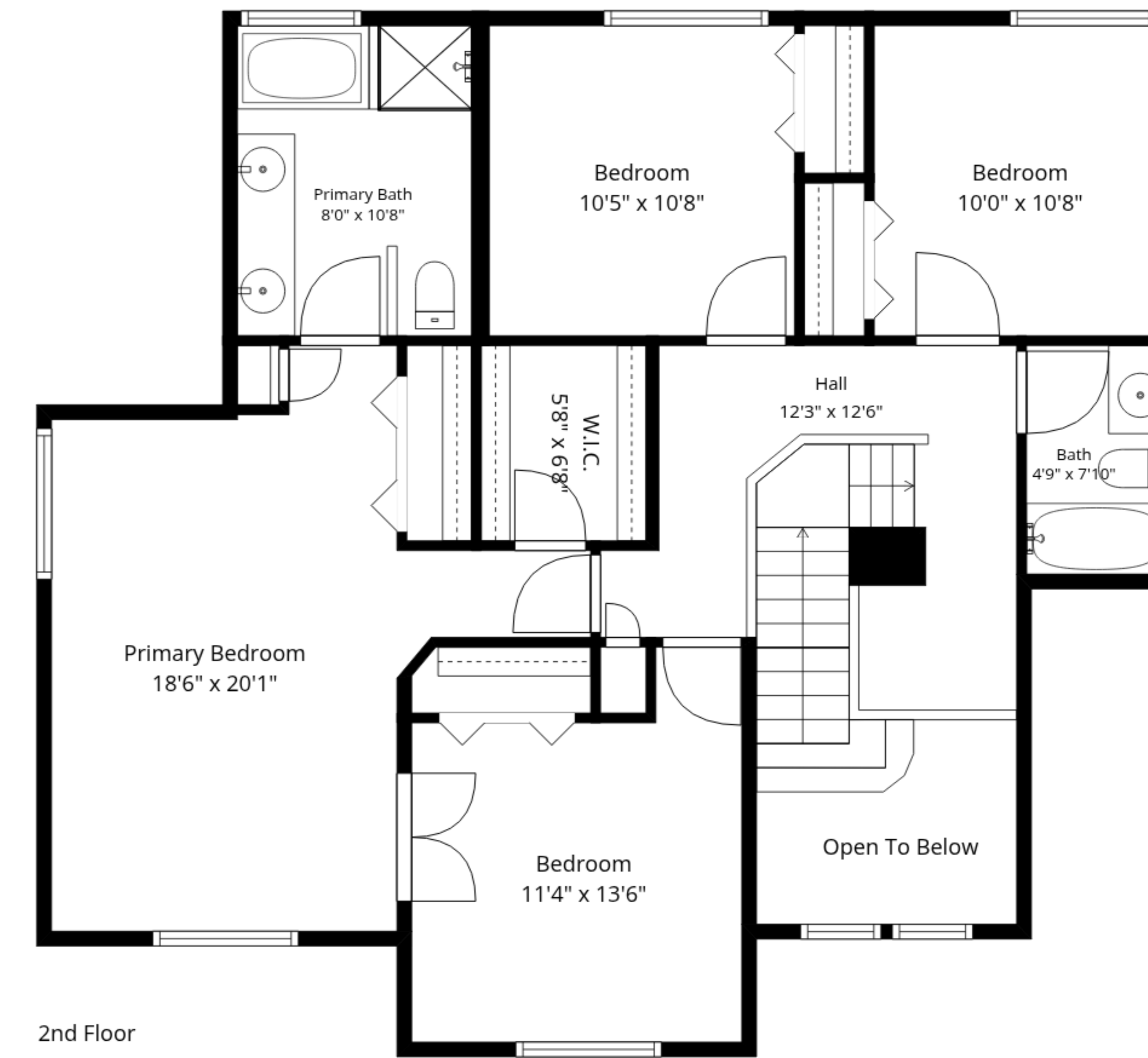
2nd Floor
