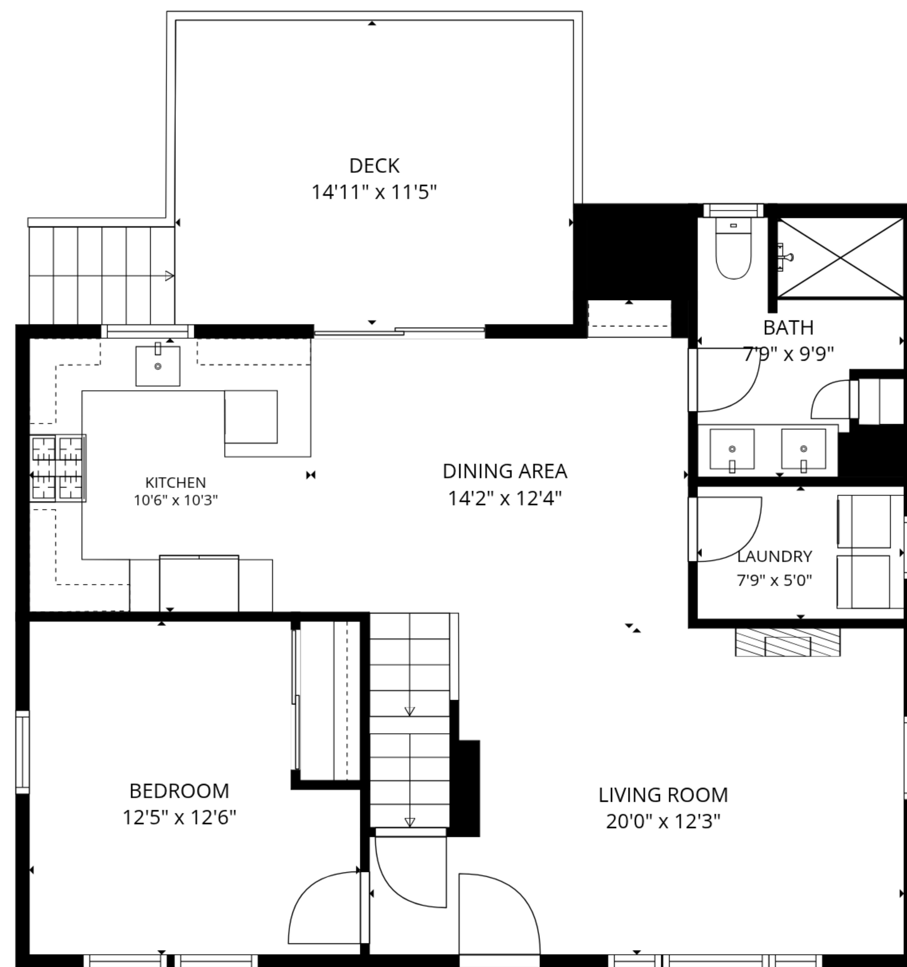
1st floor
